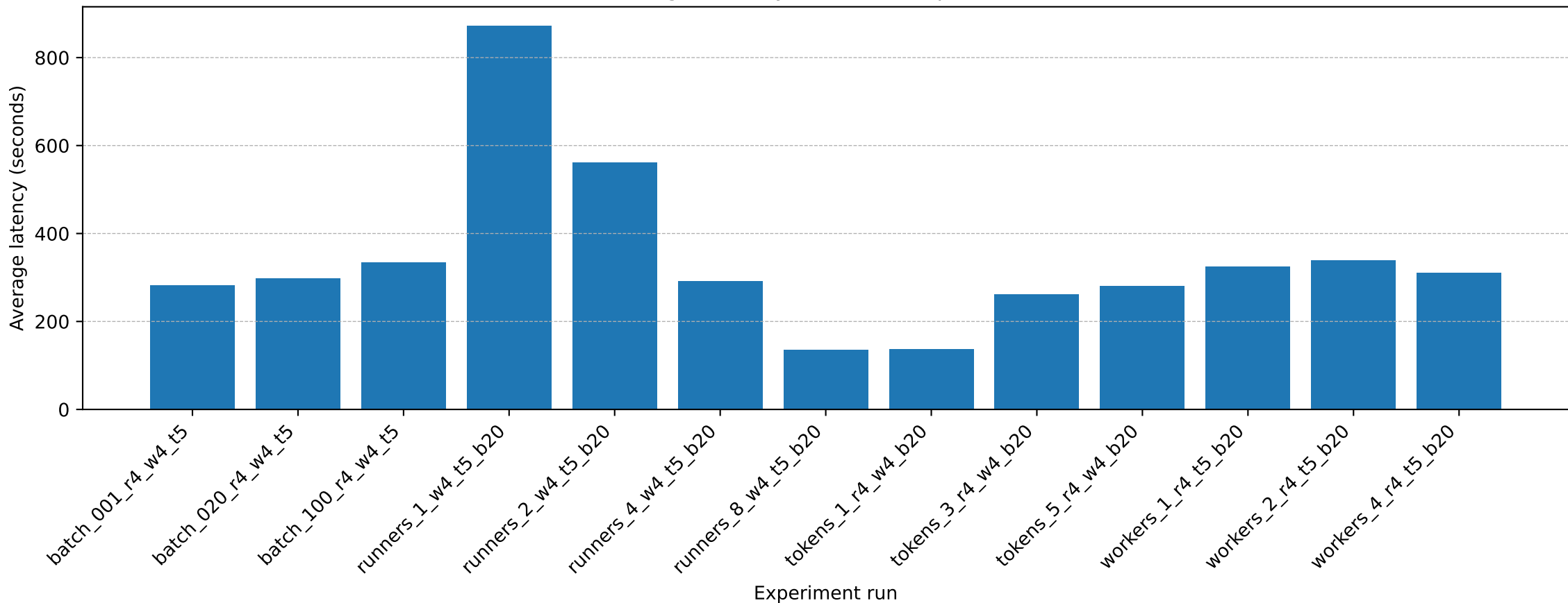
Average Latency Across All Experiments
