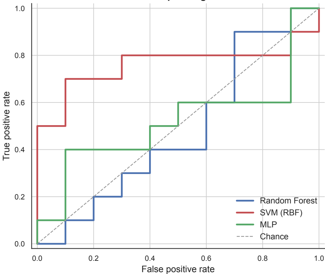
LOOCV receiver operating characteristic
