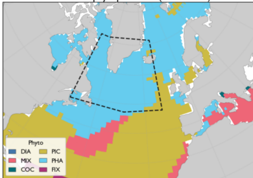
Dominant phytoplankton (2020–2024)
