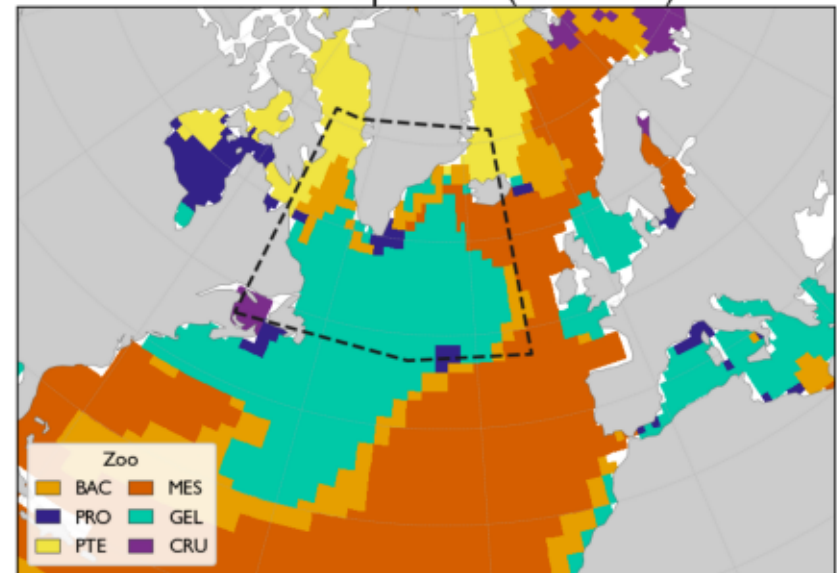
Dominant zooplankton (2020–2024)
