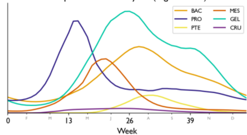
Zooplankton annual cycle (regional box)
