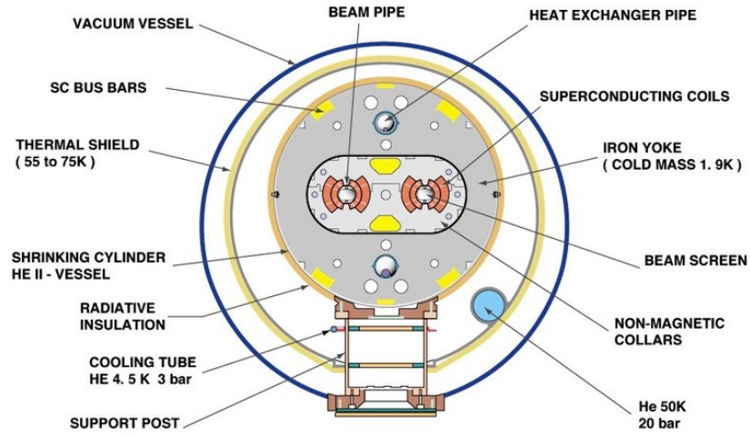
FIGURE 3.1: Cross section of the LHC cryodipole
