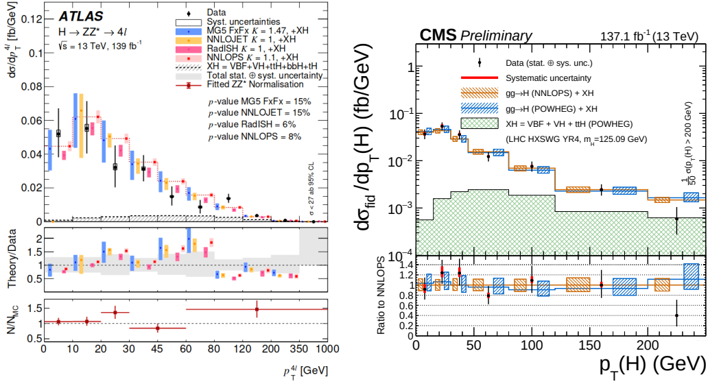
FIGURE 1.30: Left(Right): Higgs differential cross section as a function of transverse momentum of four lepton system with ATLAS (CMS) using an integrated luminosity of 139 \text{ fb}^{-1} ( 137.1 \text{ fb}^{-1} ). Results are shown with theory prediction in each experiment as described in 1.6.3.
