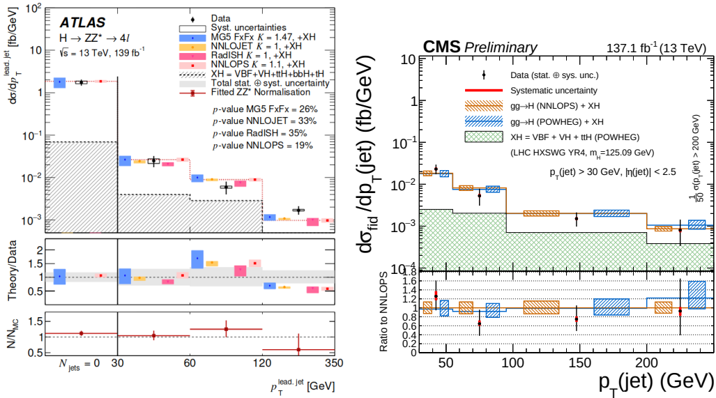
FIGURE 1.33: Left(Right): Higgs differential cross section as a function of transverse momentum of the leading jet with ATLAS (CMS) using an integrated luminosity of 139 \text{ fb}^{-1} ( 137.1 \text{ fb}^{-1} ). Results are shown with theory prediction in each experiment as described in 1.6.3.
