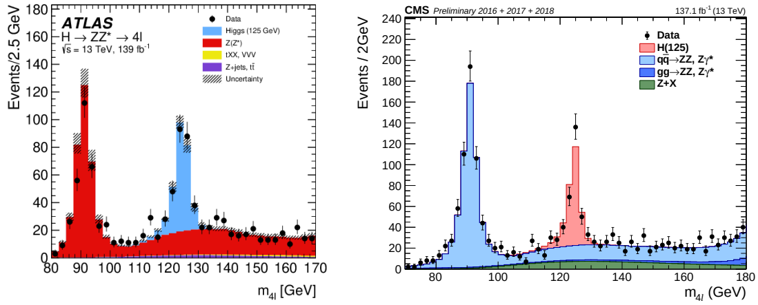
FIGURE 1.28: Left(Right): Reconstructed four-lepton invariant mass m_{4\ell} at ATLAS (CMS) using an integrated luminosity of 139 \text{ fb}^{-1} ( 137.1 \text{ fb}^{-1} ).
