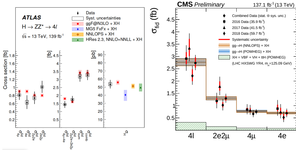
FIGURE 1.29: Left(Right): Inclusive cross section in differential final states at ATLAS (CMS) using an integrated luminosity of 139 \text{ fb}^{-1} ( 137.1 \text{ fb}^{-1} ).
