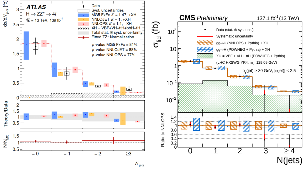
FIGURE 1.32: Left(Right): Higgs differential cross section as a function of jet multiplicity with ATLAS (CMS) using an integrated luminosity of 139 \text{ fb}^{-1} ( 137.1 \text{ fb}^{-1} ). Results are shown with theory prediction in each experiment as described in 1.6.3.
