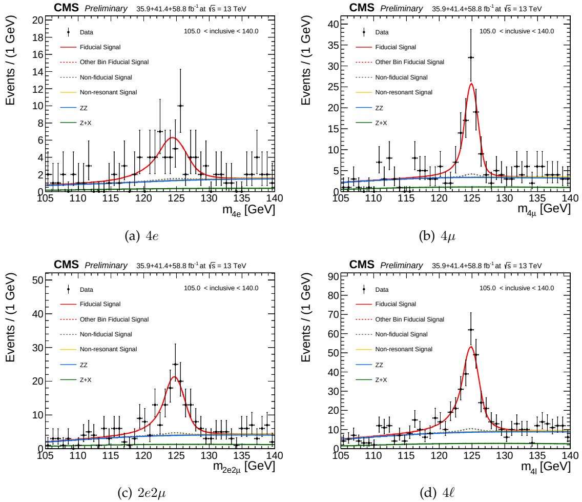
FIGURE 1.24: Inclusive four lepton invariant mass distributions in data and resulting fitted values of signal and the background PDFs in different final states.
