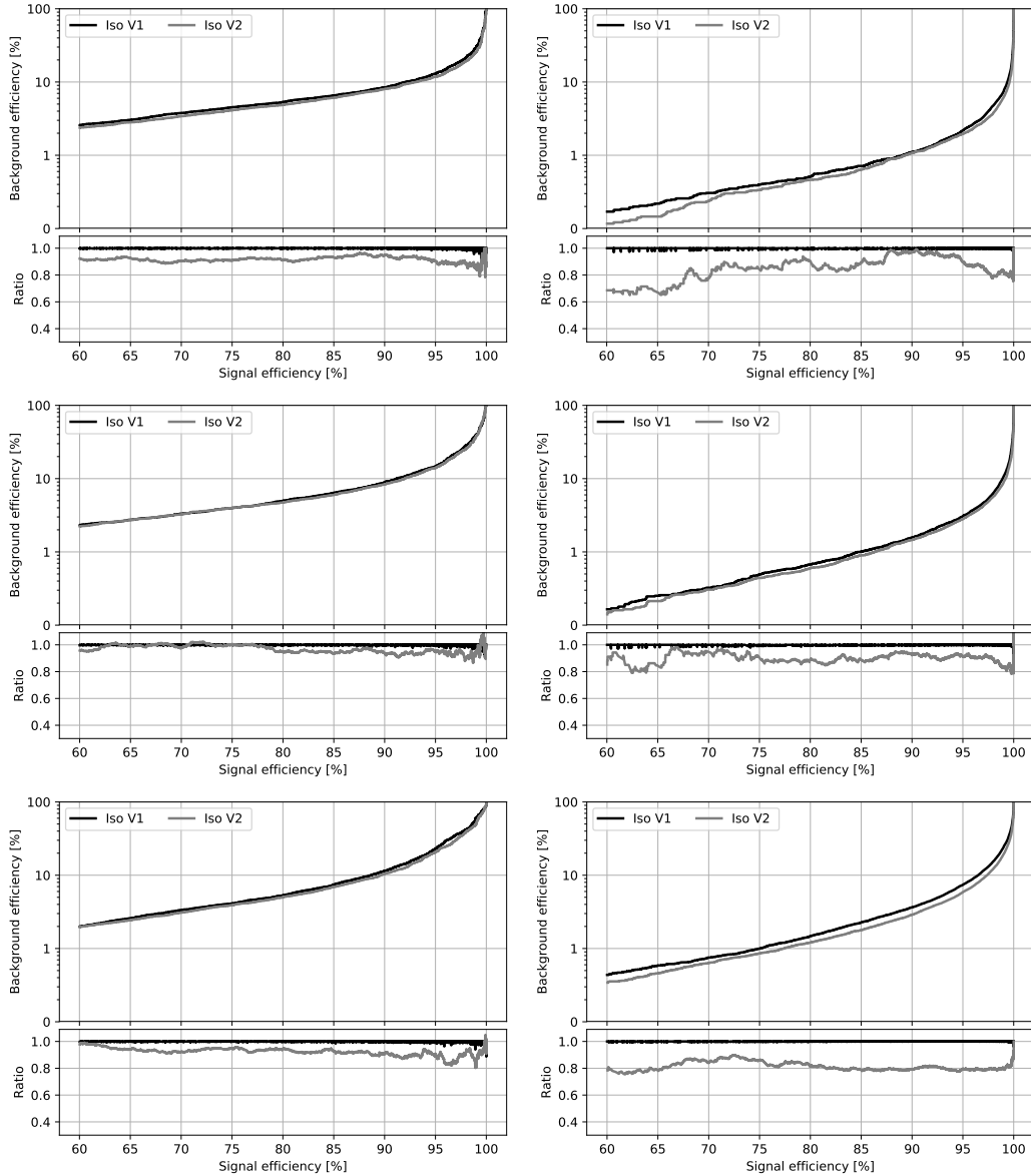
FIGURE 1.3: The receiver operating characteristic curves (background efficiency vs signal efficiency) of the MVA's trained on the 2017 simulation and applied on the 2018 simulation. The training combines identification and isolation variables. Performance are shown for electrons with 5 < p_T < 10 \text{ GeV} (left), p_T > 10 \text{ GeV} (right) and |\eta| < 0.8 (top), 0.8 < |\eta| < 1.479 (middle) and |\eta| > 1.479 (bottom). V1 and V2 versions of training are compared, exploiting TMVA and xgboost training libraries respectively.
