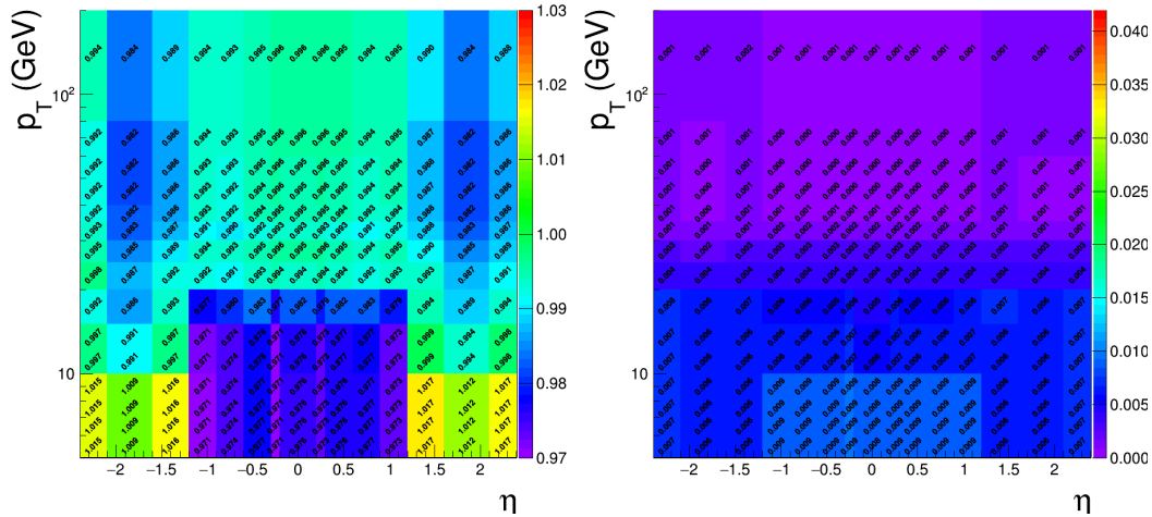
FIGURE 1.11: Left: Overall scale factors for muons, as function of p_T and \eta . Right: Uncertainties on overall scale factors muons shown in two dimensions of p_T and \eta .
