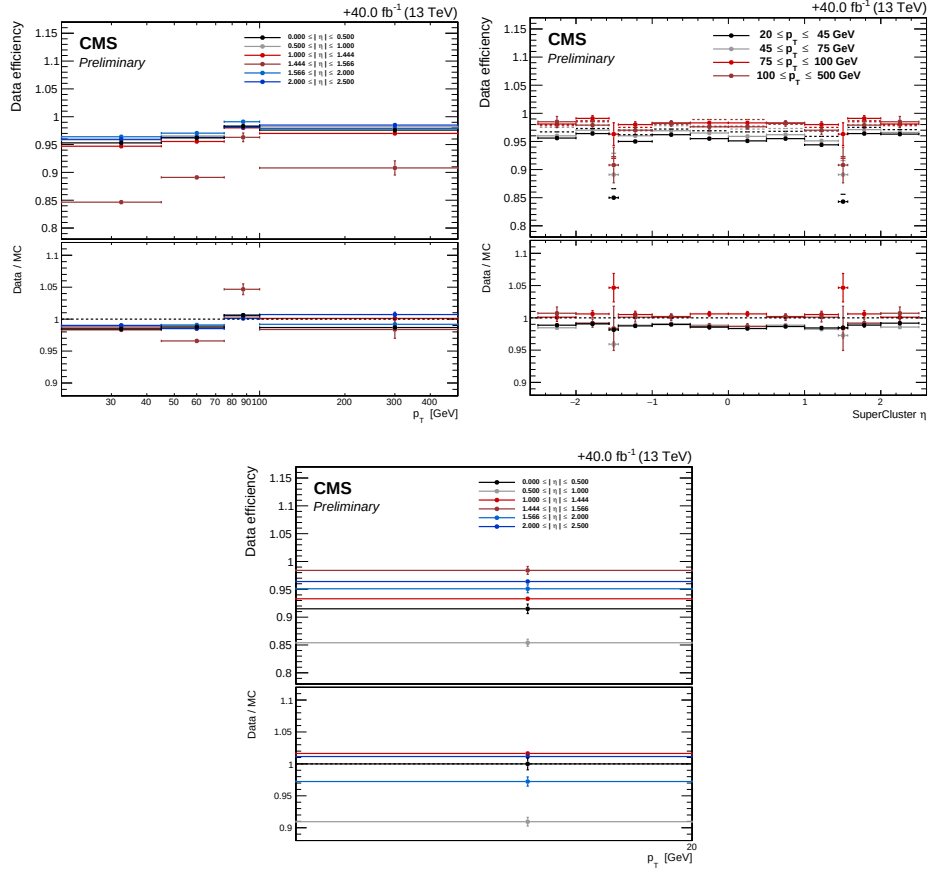
FIGURE 1.1: Reconstruction efficiencies of electron in data versus p_T (left), \eta (right) for electrons having p_T > 20 GeV (top) and p_T < 20 GeV (bottom) with corresponding data/MC scale factors as provided by the EGM POG.
