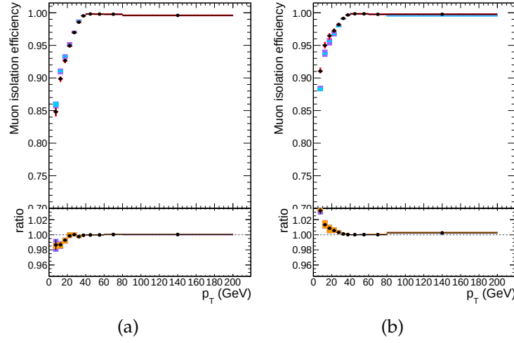
FIGURE 1.10: Efficiency of muon isolation requirement, measured with the tag&probe method on Zevents, as function of p_T in the barrel (left) and endcaps (right). In the upper panel, the larger error bars include also the systematical uncertainties, while the smaller ones are purely statistical. In the lower panel showing the ratio of the two efficiencies, the black error bars are for the statistical uncertainty, the orange rectangles for the systematical uncertainty and the violet rectangles include both uncertainties.
