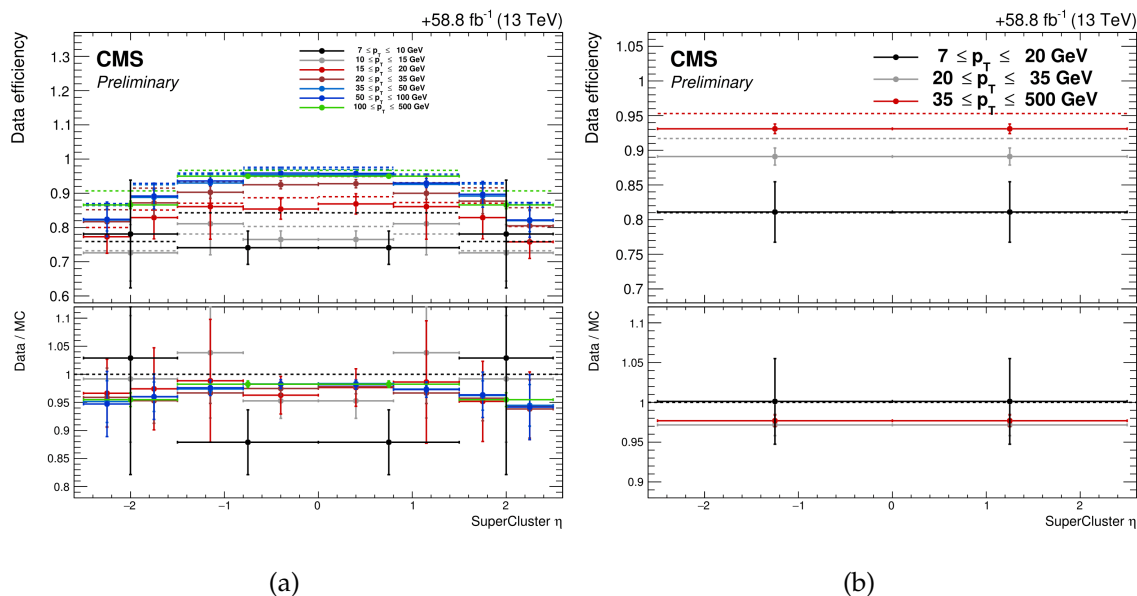
FIGURE 1.6: Electron selection efficiencies vs \eta , non-gap electrons (left) and gap electrons (right), together with the corresponding data/MC ratio at the bottom part of each plot.
