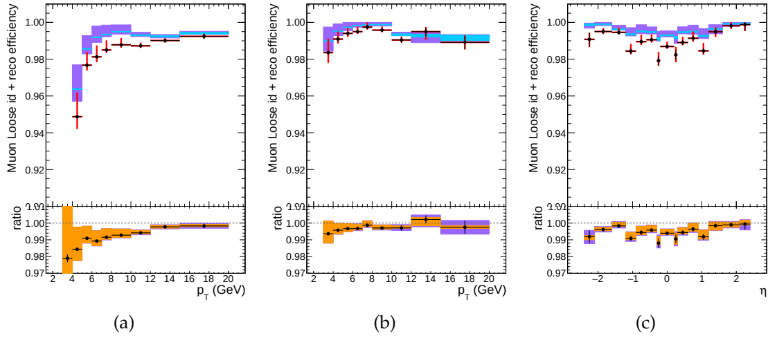
FIGURE 1.8: Reconstruction and identification efficiencies of muons at low p_T , measured with the T\&P method on events, in bins of p_T in barrel (left) and endcaps (center), and in terms of \eta for p_T > 7 GeV (right). In upper panel of each diagram, the larger uncertainty bars include also the systematical uncertainties, while the smaller ones are purely statistical. In the lower panel showing the ratio of two efficiencies, black uncertainty bars are for statistical uncertainty, the orange rectangles for the systematical uncertainty and the violet rectangles include both uncertainties.
