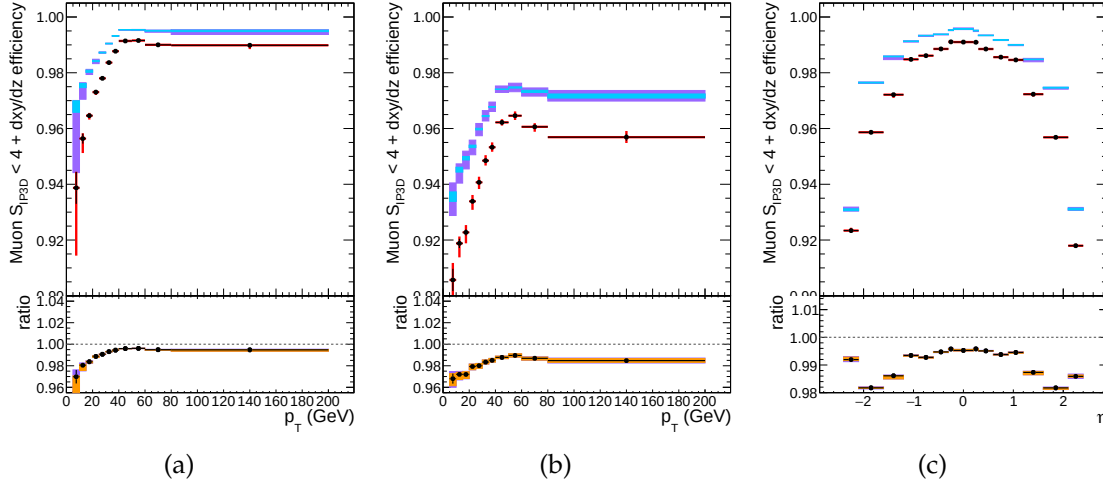
FIGURE 1.9: Efficiency of the muon impact parameter requirements, measured with the T\&P method on Z events, in bins of p_T in barrel (left) and endcaps (center), and in terms of \eta for all p_T (right). In upper panel, the larger uncertainty bars include also the systematical uncertainties, while the smaller ones are purely statistical. In the lower panel showing the ratio of two efficiencies, black error bars are for statistical uncertainty, the orange rectangles for the systematical uncertainty and the violet rectangles include both uncertainties.
