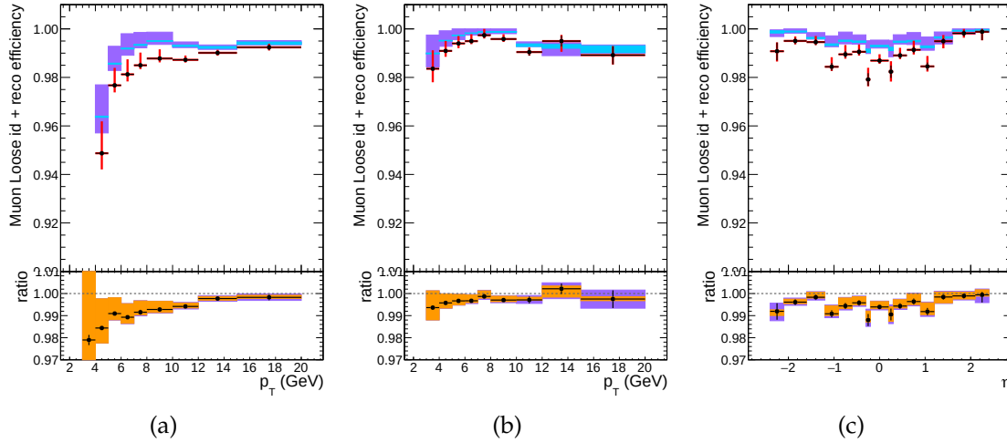
FIGURE 5.13: Reconstruction and identification efficiencies of muons at low p_T , measured with the TnP method on events, in bins of p_T in barrel (left) and endcaps (center), and in terms of \eta for p_T > 7 GeV (right). In upper panel of each diagram, the larger uncertainty bars include also the systematical uncertainties, while the smaller ones are purely statistical. In the lower panel showing the ratio of two efficiencies, black uncertainty bars are for statistical uncertainty, the orange rectangles for the systematical uncertainty and the violet rectangles include both uncertainties.
