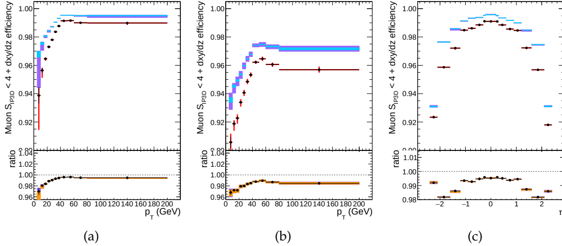
FIGURE 5.14: Efficiency of the muon impact parameter requirements, measured with the TnP method on Z events, in bins of p_T in barrel (left) and endcaps (center), and in terms of \eta for all p_T (right). In upper panel, the larger uncertainty bars include also the systematical uncertainties, while the smaller ones are purely statistical. In the lower panel showing the ratio of two efficiencies, black error bars are for statistical uncertainty, the orange rectangles for the systematical uncertainty and the violet rectangles include both uncertainties.
