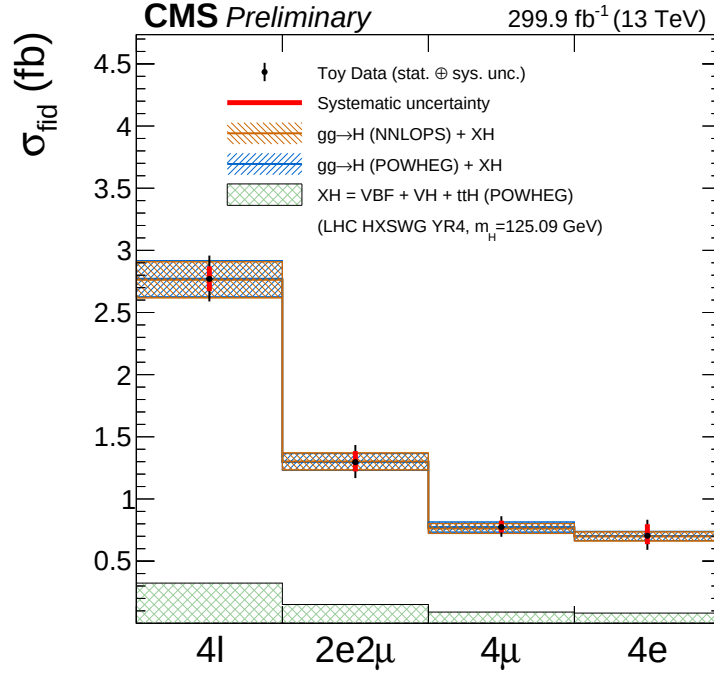
FIGURE 7.2: Expected Higgs inclusive cross section at 300 \text{ fb}^{-1}
