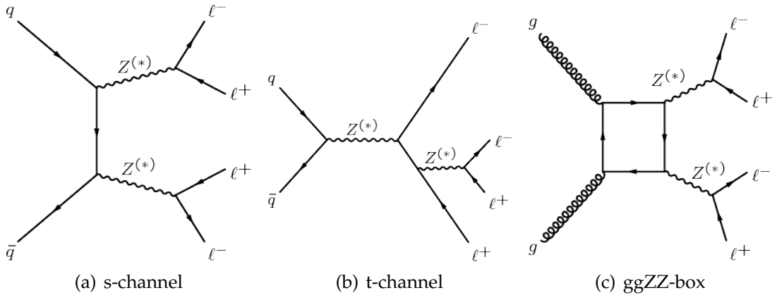
FIGURE 6.4: q\bar{q}toZZ \rightarrow 4\ell process s- and t- channel fynman diagrams (a) and (b). gg \rightarrow ZZ \rightarrow 4\ell process fynman diagram (c).
