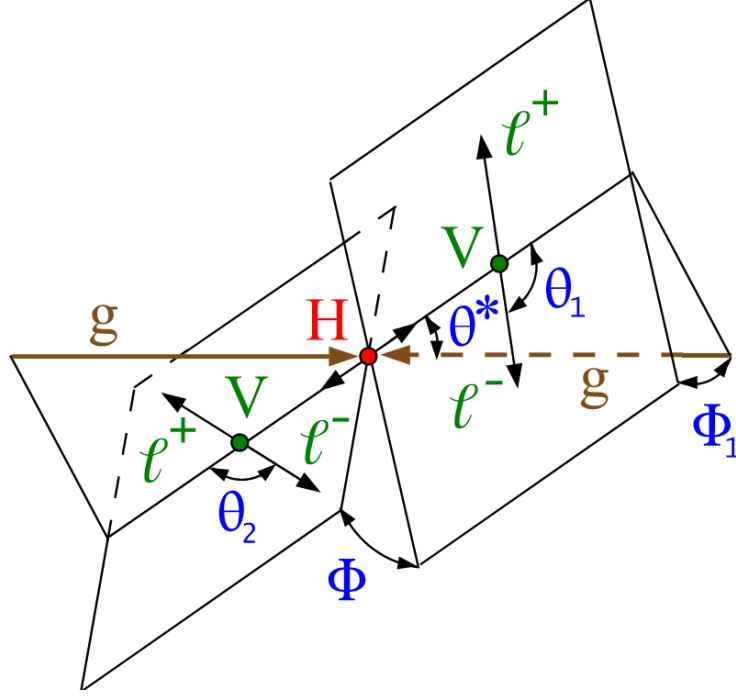
FIGURE 7.1: Higgs event signature
