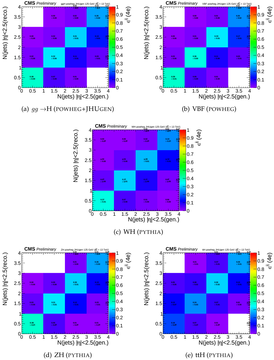
FIGURE 8.21: Efficiency matrices for N(jets) for different SM production modes in the 4e final state.
