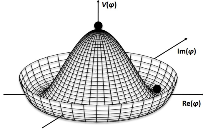
FIGURE 2.2: The Higgs potential as in Eq.??
