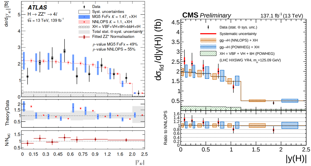
FIGURE 6.31: Left(Right): Higgs differential cross section as a function of rapidity of four lepton system with ATLAS (CMS) using an integrated luminosity of 139 \text{ fb}^{-1} ( 137.1 \text{ fb}^{-1} ). Results are shown with theory prediction in each experiment as described in ??.
