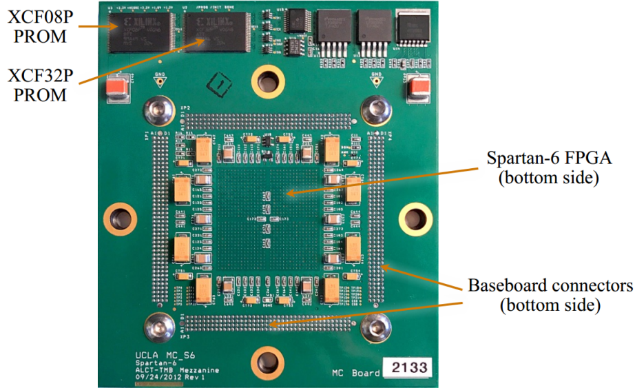
FIGURE 1.3: The Spartan-6 ALCT mezzanine boards produced for the ME1/1 upgrade which will be around 104\text{mm} \times 140\text{mm} to accommodate the new optical components.
