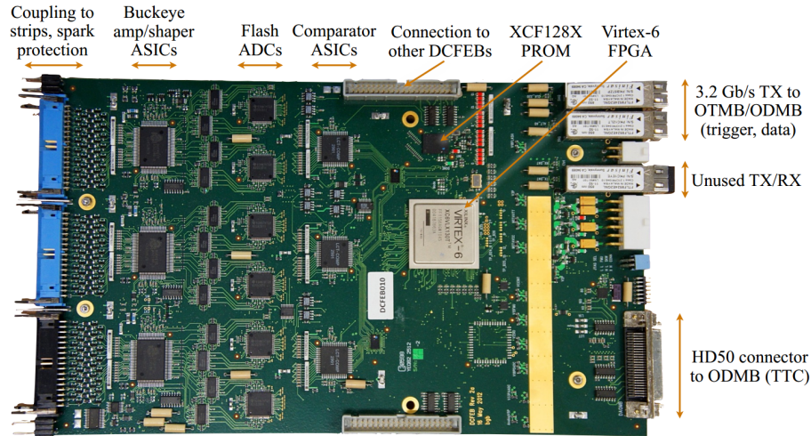
FIGURE 1.2: One of the DCFEB used for ME1/1.
