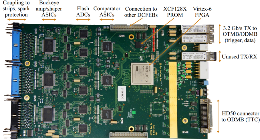
FIGURE 1.2: One of the DCFEBs used for ME1/1.
