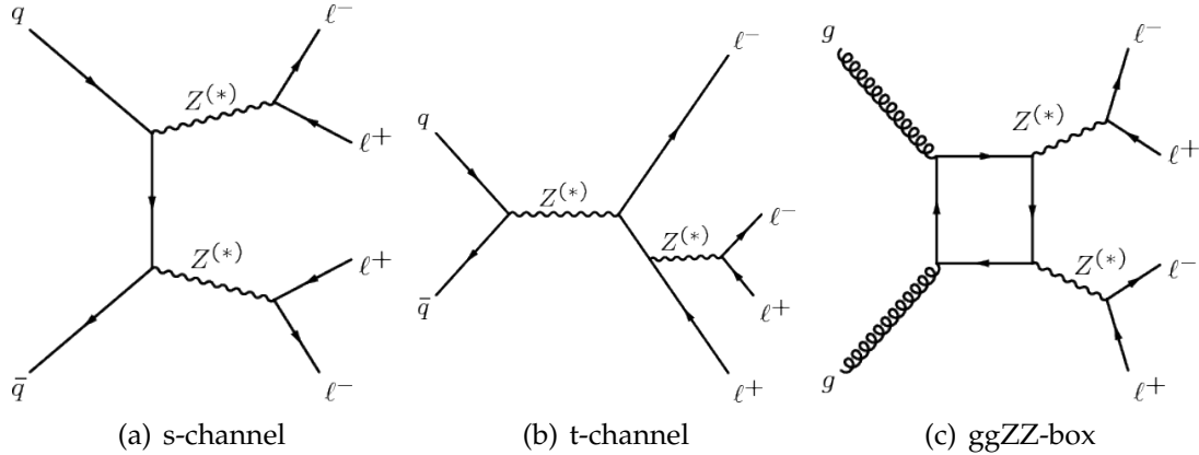
FIGURE 6.4: q\bar{q} \rightarrow ZZ \rightarrow 4\ell process s- and t- channel fynman diagrams (a) and (b). gg \rightarrow ZZ \rightarrow 4\ell process fynman diagram (c).
