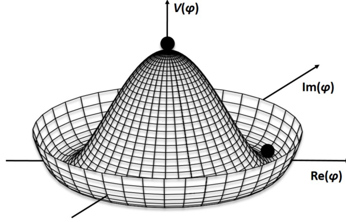
FIGURE 1.2: The Higgs potential as in Eq.1.6
