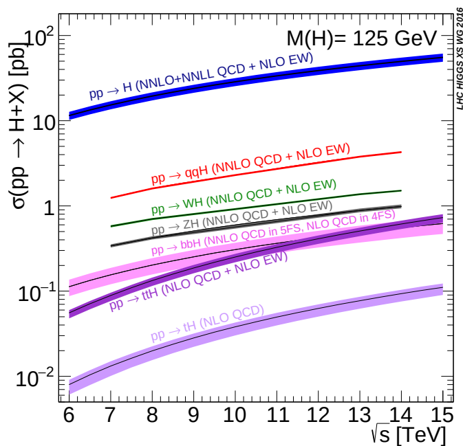
FIGURE 1.5: Production cross sections of Higgs boson ( m_H = 125 GeV) as a function of center of mass energies
