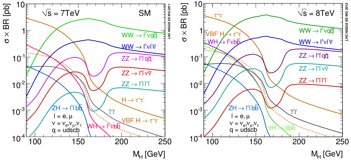
FIGURE 1.7: Cross sections of Higgs times branching ratios at 7 TeV and 8 TeV (left and right diagrams respectively).
