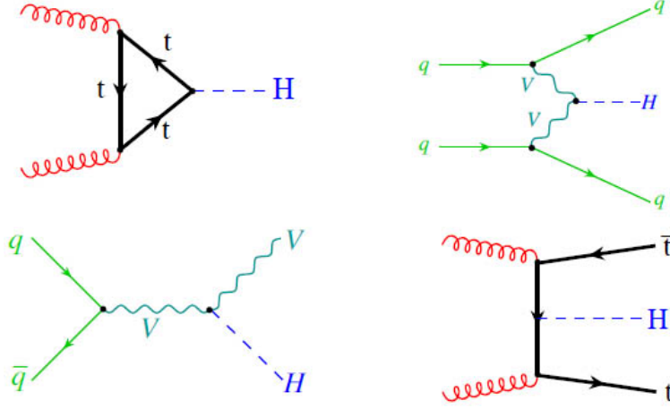
FIGURE 1.3: Feynman diagrams of Higgs production at tree level: gluon-gluon fusion (upper left); VV fusion (upper right); associated production with W and Z bosons (bottom left); associated production with t\bar{t} (bottom right).
