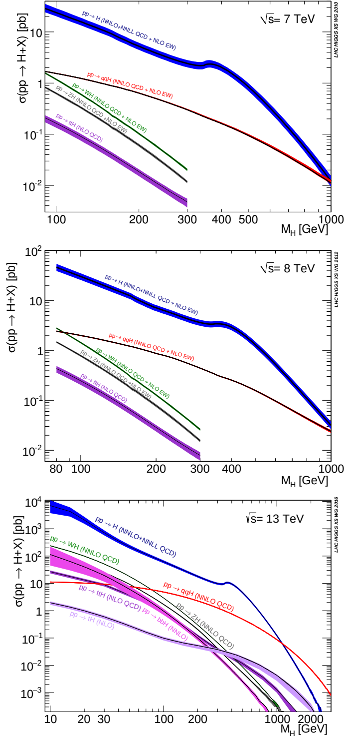
FIGURE 1.4: Production cross sections of SM Higgs boson at 7, 8 and 13 TeV as function of its mass.
