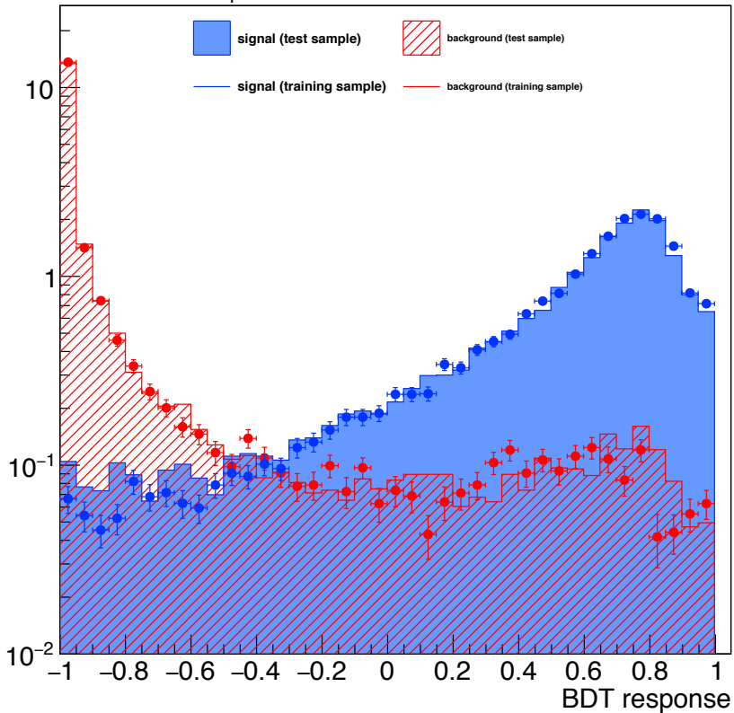
barrel I, 5 < p_T < 10 GeV
