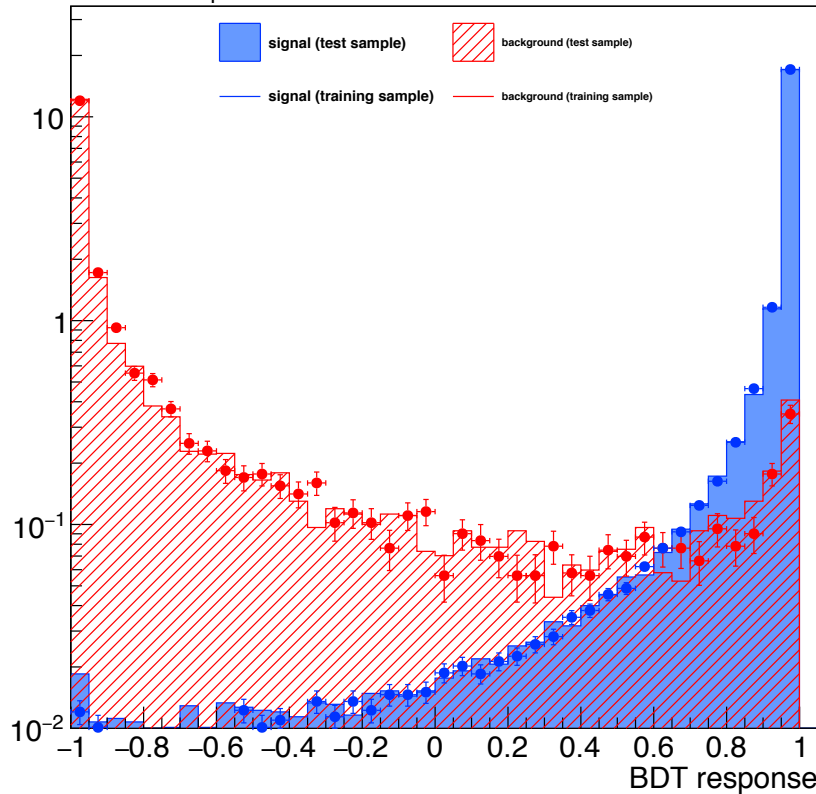
barrel I, p_T > 10 GeV
