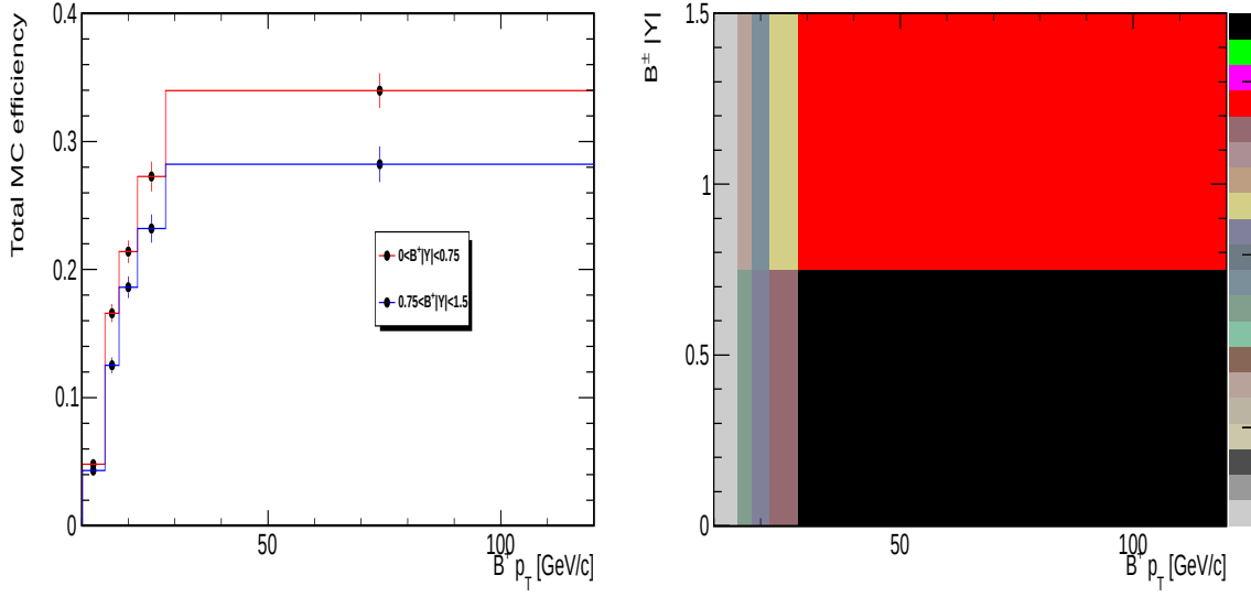
Figure 32: \epsilon_{MC} of B^+ \rightarrow J/\psi K^+ for 2D candidates in different p_T and |y| bins.
