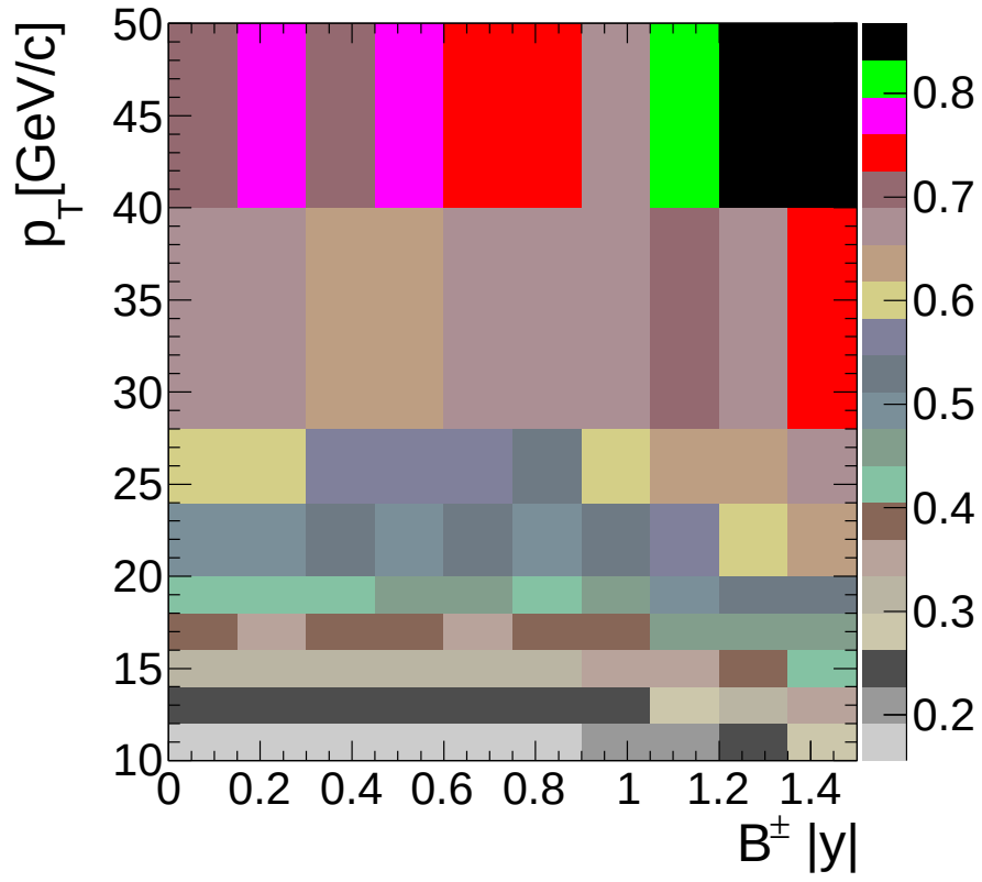
Figure 15: The acceptance of B^\pm \rightarrow J/\psi K^\pm , J/\psi \rightarrow \mu^+ \mu^- process in B^\pm p_T and |y| dimensions.
