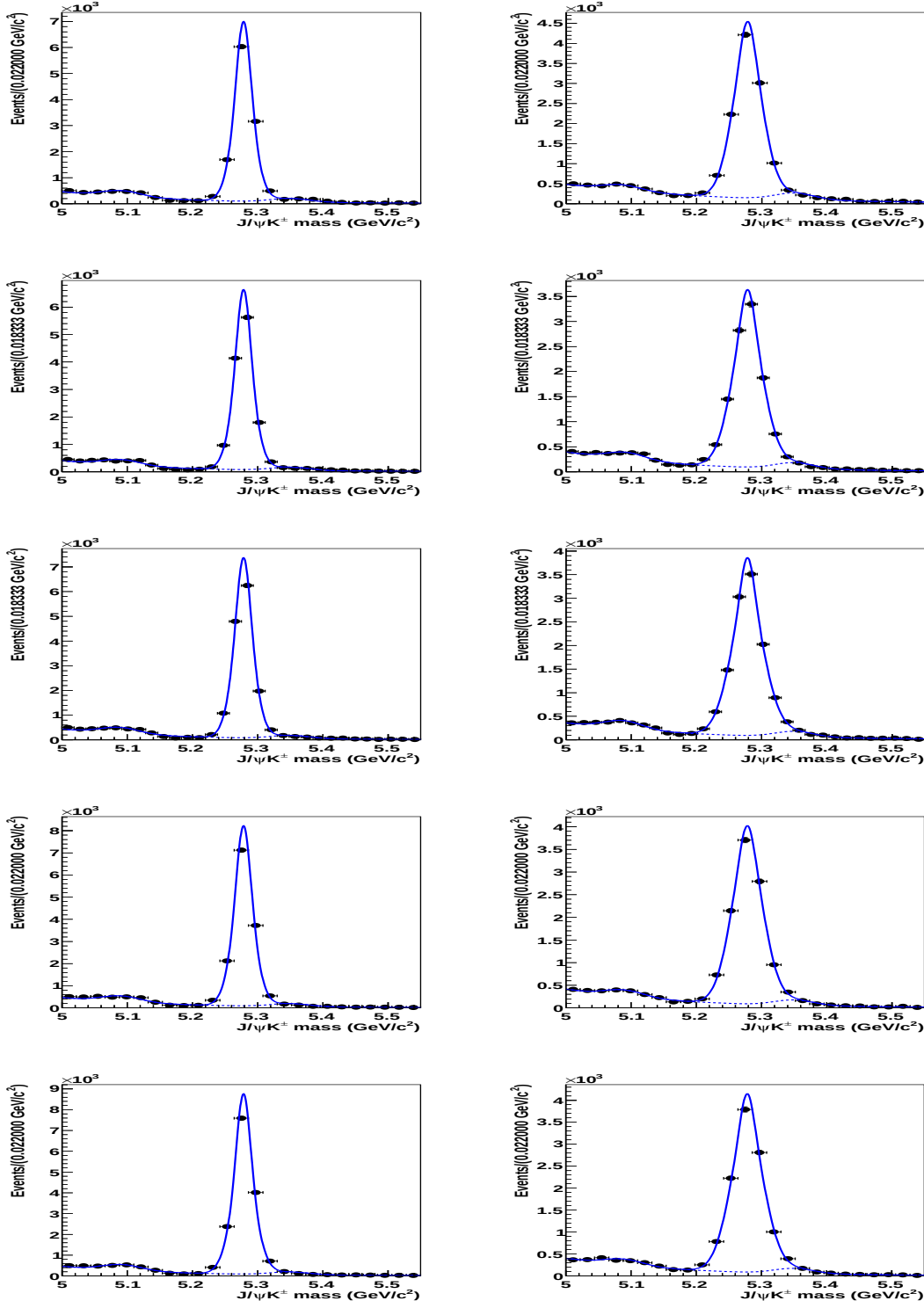
Figure 31: Mass fit plots of J/\psi K^\pm 2D candidates. left: for small rapidity 0.0 < |y| < 0.75 , right: for large rapidity 0.75 < |y| < 1.5 , top to bottom is for the five p_T differential bins of B^\pm .
