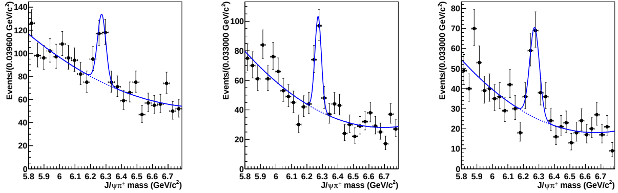
Figure 8: From left to right, fits to the inv. mass distributions of J/\psi and \pi in data for B_c p_T bins 10-16, 16-22 and >22 \text{ GeV}/c .
