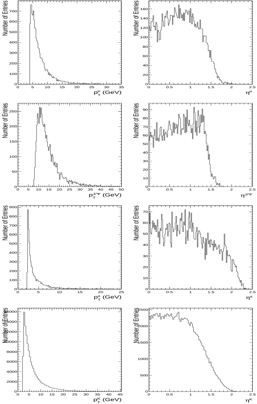
Figure 2: Distributions of p_T and |\eta| of muons, J/\psi 's, pions and kaons after final selections in data.
