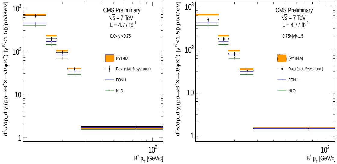
Figure 39: 2D ( p_T - |y| ) differential production cross sections for B^+ \rightarrow J/\psi K^+ at \sqrt{s} = 7 TeV pp collision left: for 0.0 < |y| B^+ < 0.75 , right: for 0.75 < |y| B^+ < 1.5 . Dots with uncertainties are the CMS measurement, uncertainties are systematics and statistics uncertainties respectively. The color bands covers the PYTHIA predictions whereas the width of bands involve the error arising due to the error of PYTHIA for Br(B^\pm \rightarrow J/\psi K^\pm) of 1.014 \times 10^{-3} \pm 3.4 \times 10^{-5} in PDG [51]. The theoretical predictions of NLO and FONLL has also been added where the error is the fraction of b\bar{b} \rightarrow B^\pm + X ( 0.337 \pm 0.020 ) and of Br(B^\pm \rightarrow J/\psi K^\pm) to be 1.014 \times 10^{-3} \pm 3.4 \times 10^{-5} .
