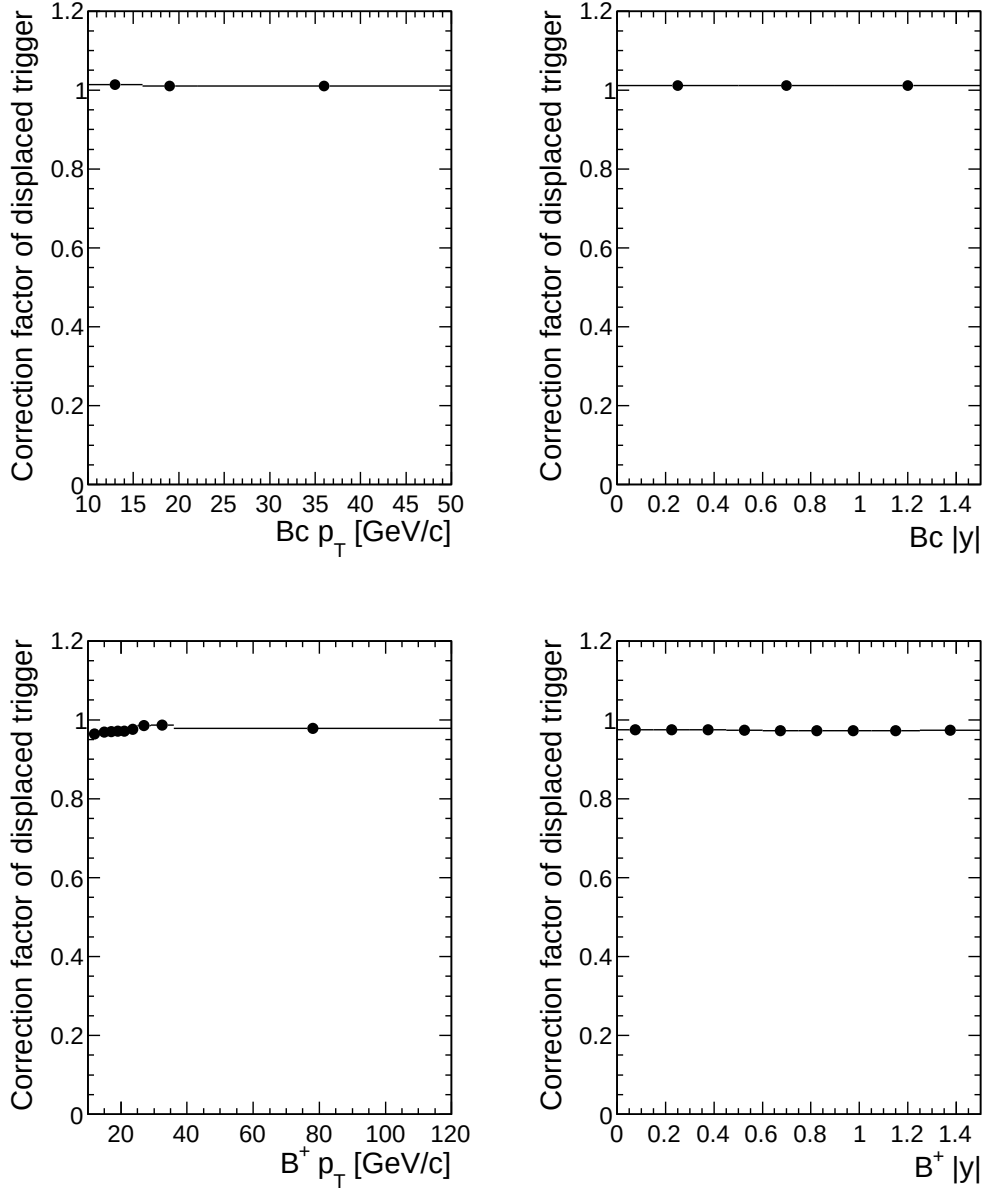
Figure 27: The correction factor \alpha_{Disp} for different B_c (top) and B^\pm (bottom) p_T and |y| bins.
