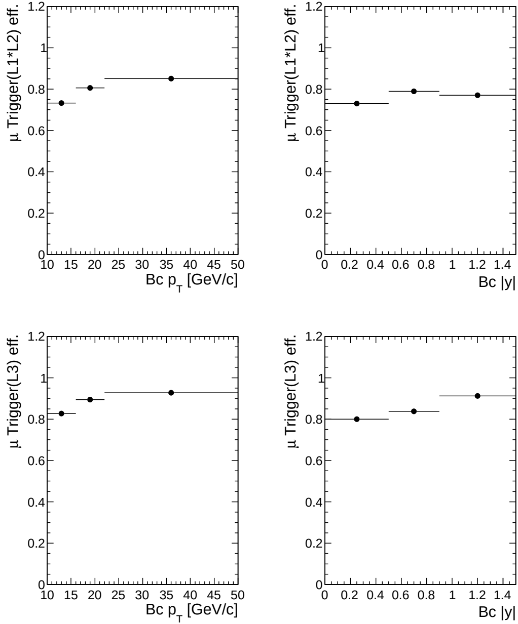
Figure 20: Efficiencies of trigger L1 \cdot L2 (top) and L3 (bottom) as a function of B_c p_T (left) and y (right). Dimuon efficiency is computed from the product of the two single muons efficiencies.
