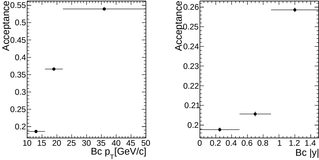
Figure 14: B_c acceptance as a function of B_c p_T (left) and rapidity (right), where the uncertainties reflect the MC statistics.
