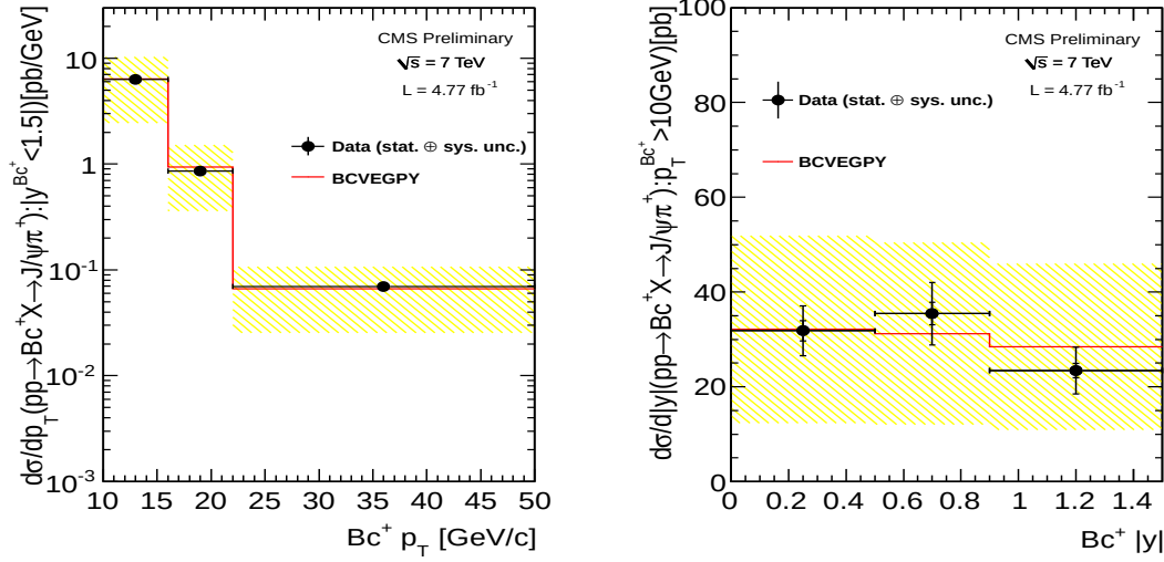
Figure 37: Differential production cross sections of d\sigma/dp_T^{B_c^+ \rightarrow J/\psi \pi^+} and d\sigma/d|y|^{B_c^+ \rightarrow J/\psi \pi^+} at \sqrt{s} = 7 TeV pp collisions. Dots with uncertainties bars are the CMS measurements, uncertainties are systematical uncertainties and statistic uncertainties respectively. Red histogram is BCVEGPY prediction. The uncertainties of BCVEGPY is branching ratio uncertainties of the Br(B_c \rightarrow J/\psi \pi) which is 1.3 \times 10^{-03} \pm 8.0 \times 10^{-04} in reference [53].
