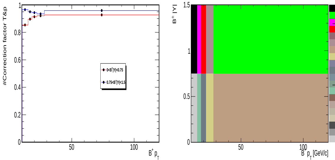
Figure 35: \alpha_{T-P} of B^+ \rightarrow J/\psi K^+ for 2D candidates in different p_T and |y| bins.
