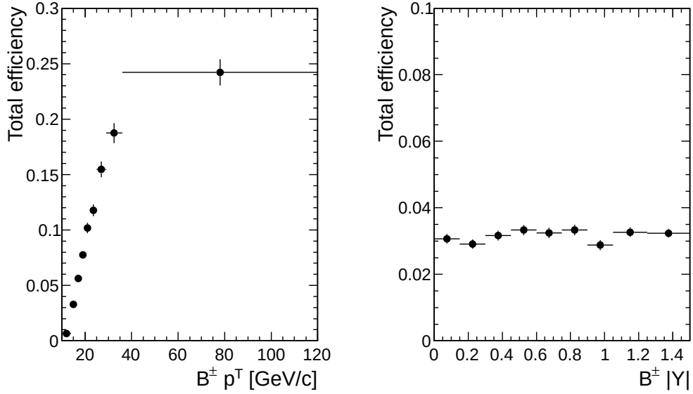
Figure 29: Total efficiency \epsilon = Acc. \cdot \epsilon_{MC} \cdot \alpha_{2\mu} \cdot \alpha_{Disp} , as a function of B^\pm p_T (left) and rapidity (right).
