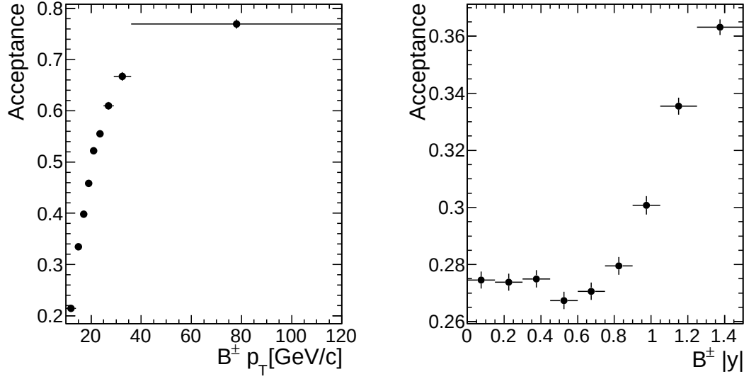
Figure 16: B^\pm \rightarrow J/\psi(\mu^+\mu^-)K^\pm acceptance as a function of B^\pm p_T (left) and absolute rapidity |y| (right), where the uncertainties reflect the MC statistical uncertainties.
