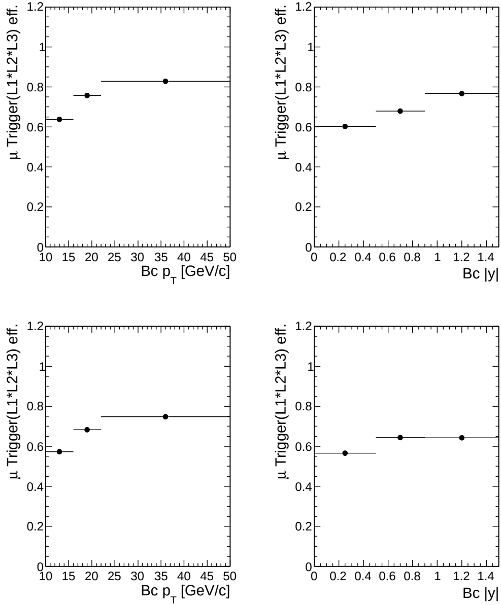
Figure 19: L1.L2.L3 trigger efficiencies as a function of B_c p_T (left) and |y| (right) for seagulls (top) and cowboys (bottom) muons. In each case, dimuon efficiency is computed from the product of the two single muon efficiencies.
