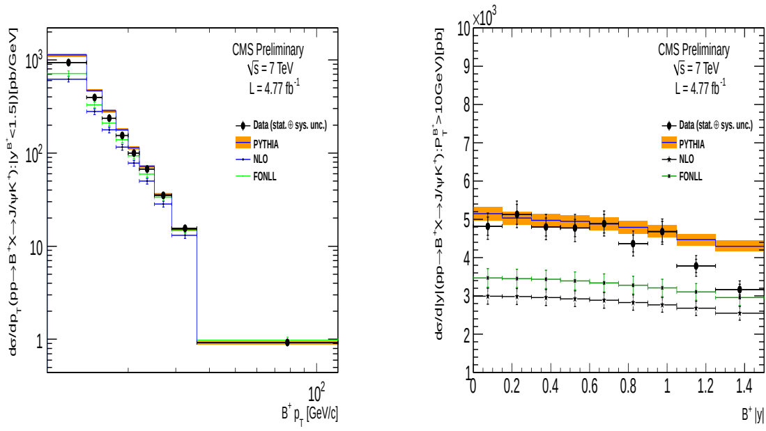
Figure 38: Differential production cross sections of d\sigma/dp_T^{B^+ \rightarrow J/\psi K^+} and d\sigma/d|y|^{B^+ \rightarrow J/\psi K^+} at \sqrt{s} = 7 TeV pp collisions. Dots with uncertainties are the CMS measurements, uncertainties are systematical uncertainties and statistical uncertainties respectively. The color bands are PYTHIA predictions. The uncertainties of PYTHIA are branching ratio uncertainties of the Br(B^\pm \rightarrow J/\psi K^\pm) which is 1.014 \times 10^{-03} \pm 3.4 \times 10^{-05} in PDG [51].
