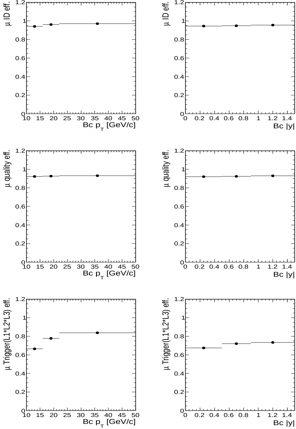
Figure 21: Efficiencies as a function of B_c p_T (left) and |y| (right) for muon identification (top), muon quality (middle) and trigger ( L1 \cdot L2 \cdot L3 ) (bottom) for the B_c MC samples.
