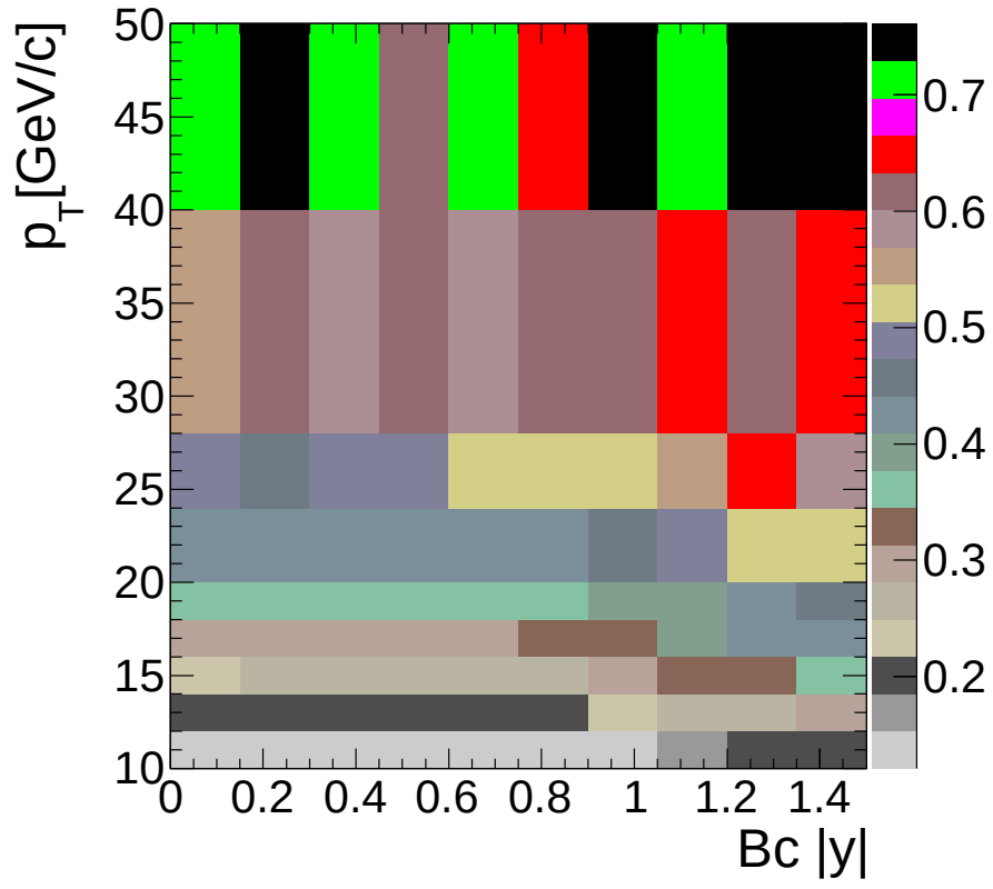
Figure 13: The acceptance of B_c \rightarrow J/\psi \pi , J/\psi \rightarrow \mu^+ \mu^- process in B_c p_T and |y| dimensions.
