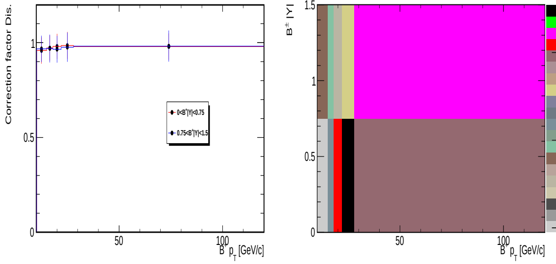
Figure 34: \alpha_{Disp-trigger} of B^+ \rightarrow J/\psi K^+ for 2D candidates in different p_T and |y| bins.
