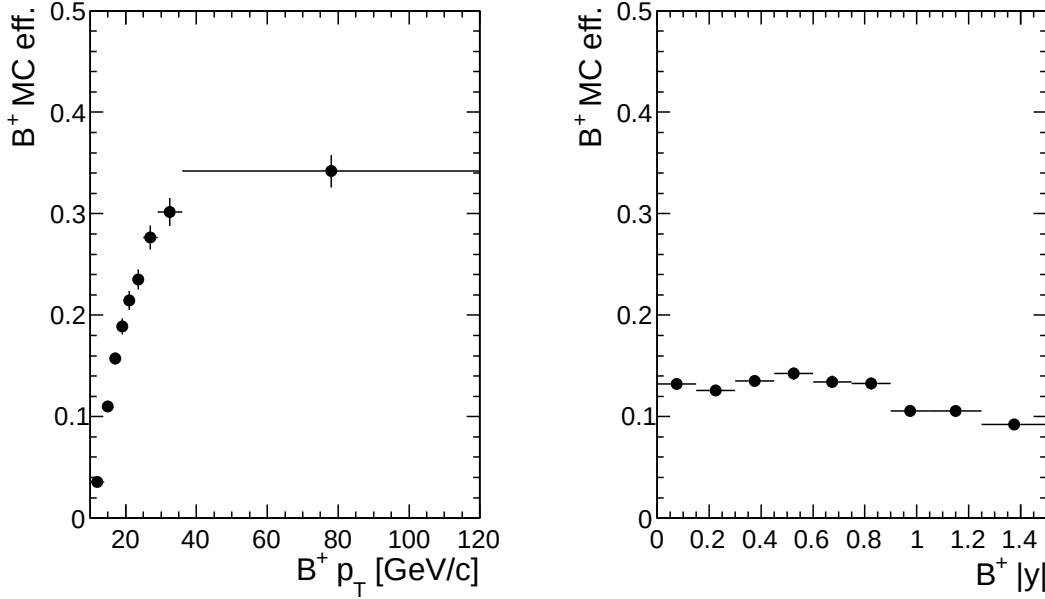
Figure 18: The MC efficiency \epsilon_{MC} for different B^\pm p_T (left) and |y| (right) bins.
