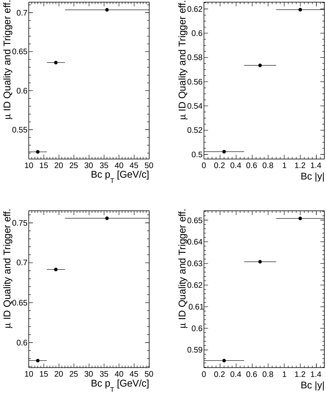
Figure 23: Dimuon efficiencies as a function of B_c p_T (left) and |y| (right). Upper plots are for the data and lower plots are for the MC samples.
