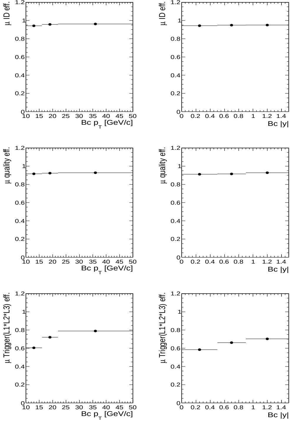
Figure 22: Efficiencies as a function of B_c p_T (left) and |y| (right) for muon identification (top), muon quality cuts (middle) and the Trigger ( L1 \cdot L2 \cdot L3 ) (bottom) for the data.
