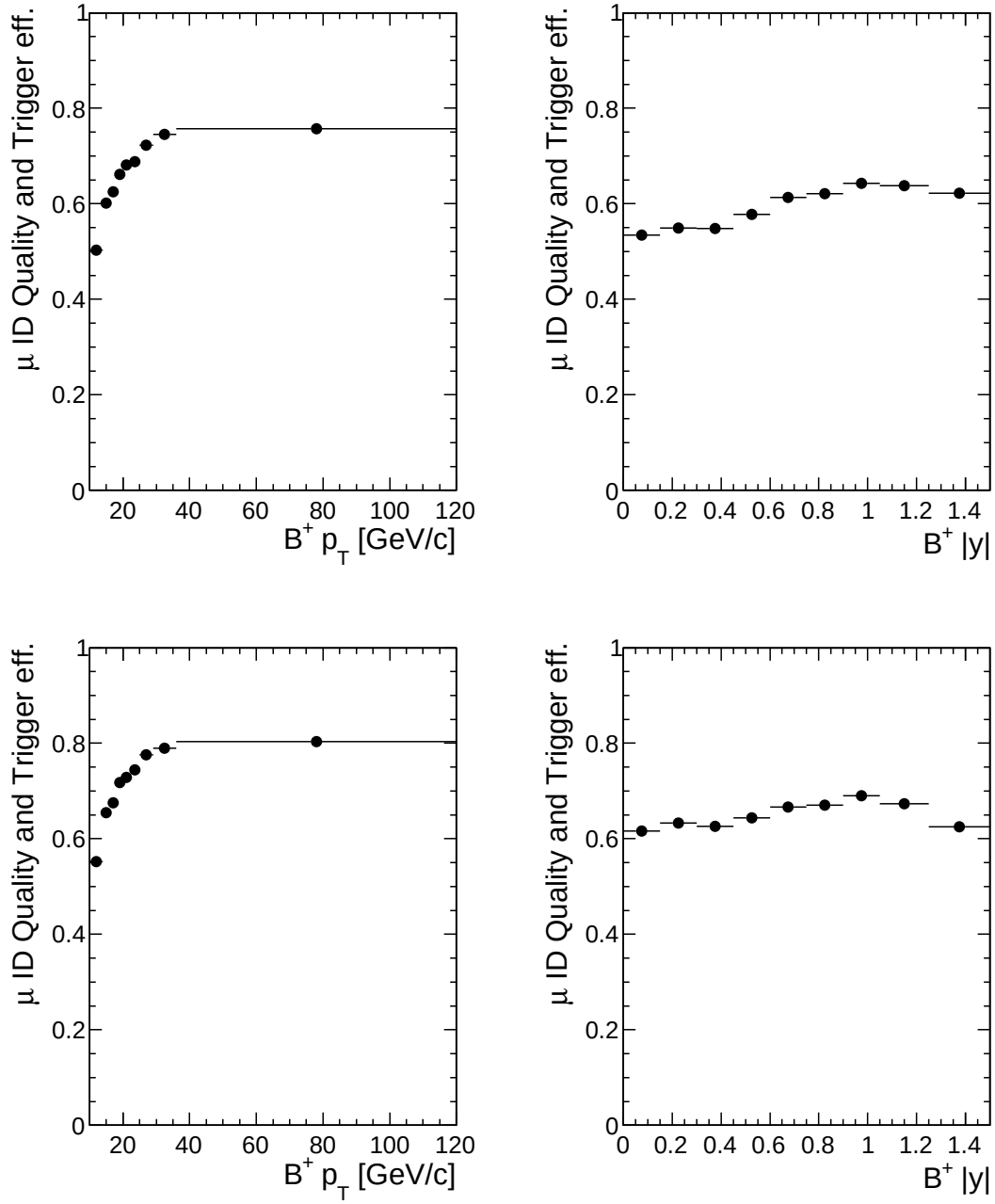
Figure 25: Dimuon efficiencies as a function of B^\pm p_T (left) and |y| (right). Upper plots are for the data and lower plots are for the MC samples.
