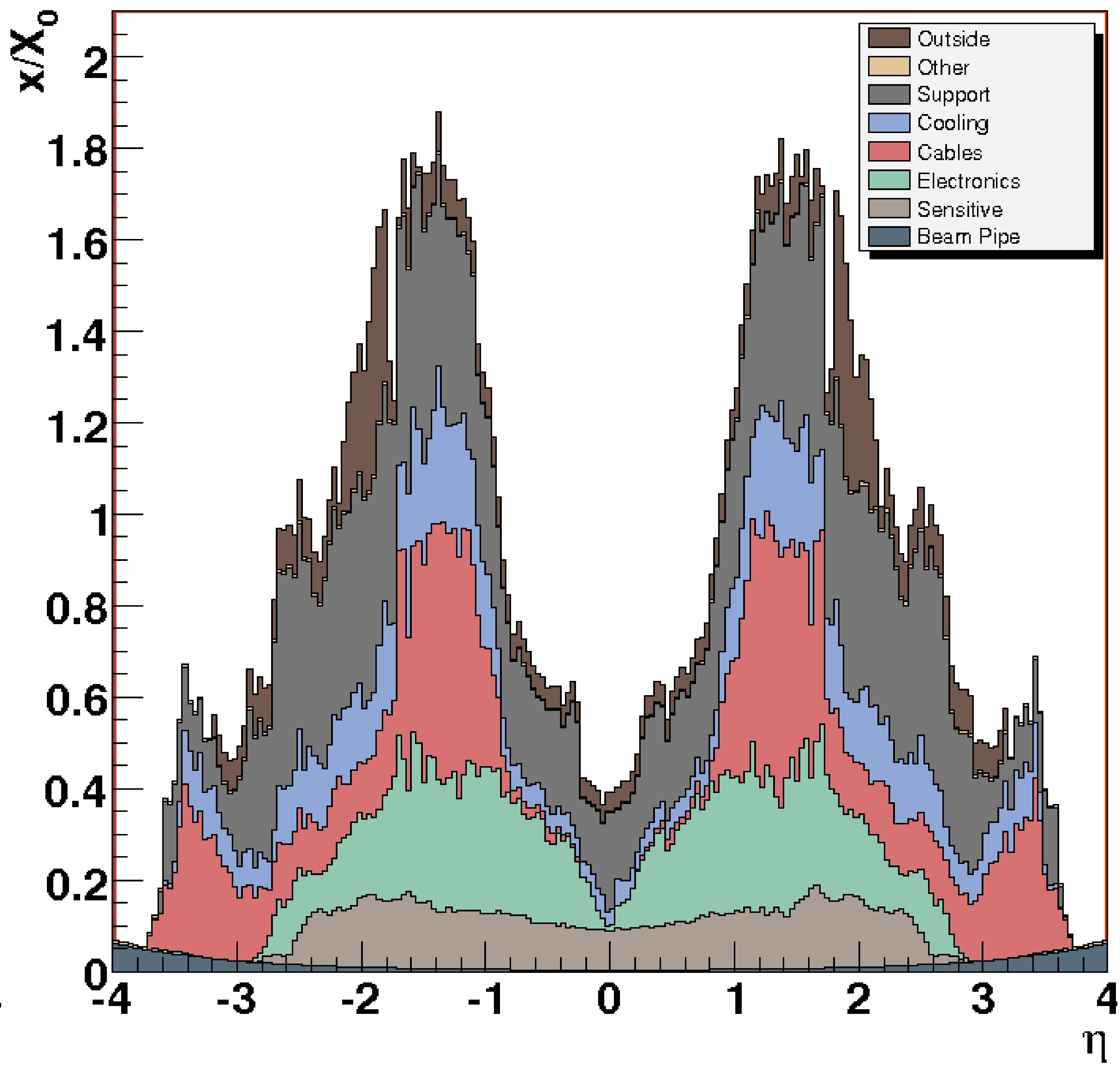
Tracker Material Budget
