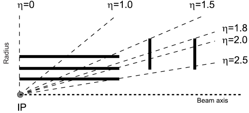
FIGURE 3.8: CMS pixel detectors and hit coverage. Lines represent detector modules [42].
