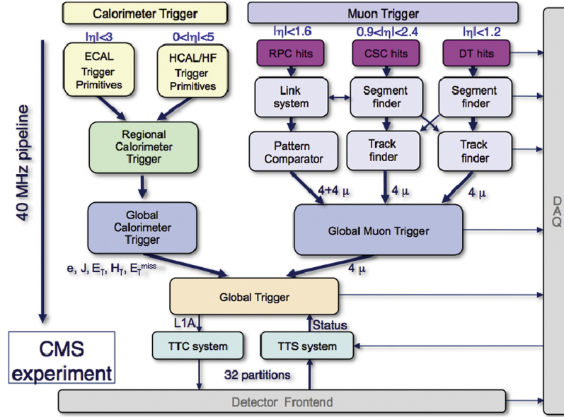
FIGURE 3.19: The configuration of L1 trigger.
