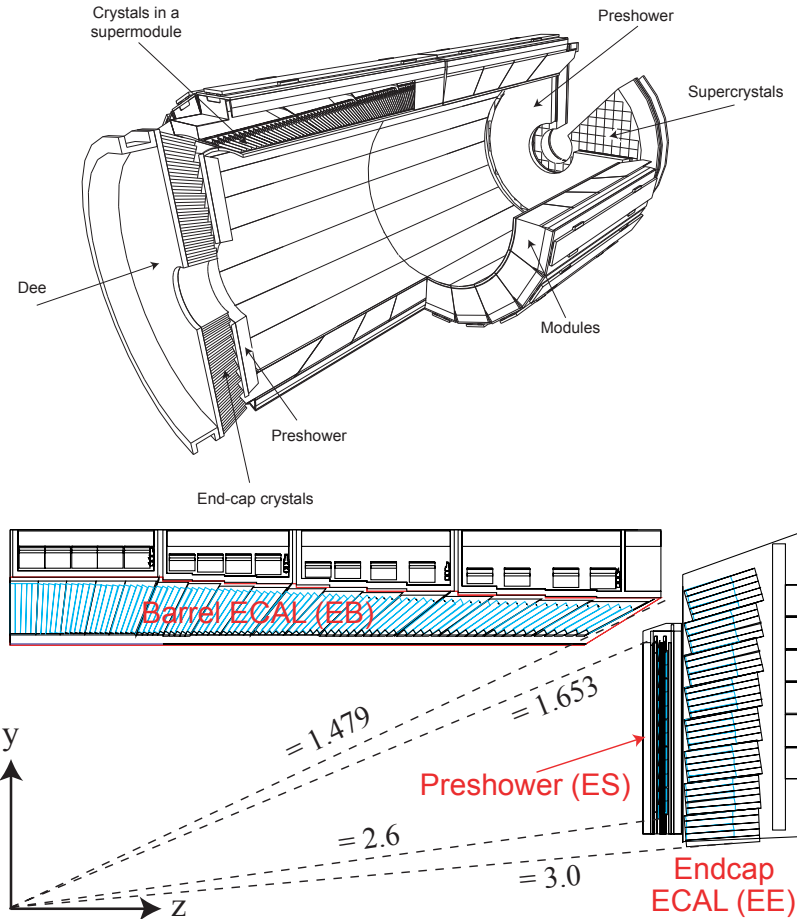
FIGURE 3.12: CMS ECAL layout and pseudorapidity coverage [42].
