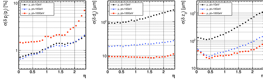
FIGURE 3.10: Expected single muons tracks resolution of transverse momentum (left), transverse impact parameter (middle) and longitudinal impact parameter (right) of p_T = 1, 10, 100 GeV [42].
