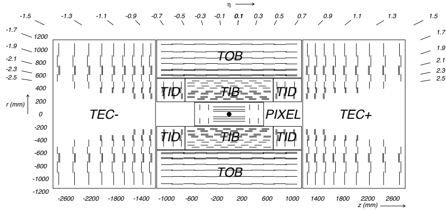
FIGURE 3.7: Schematic diagram of CMS tracker system. Lines represent detector modules [42].
