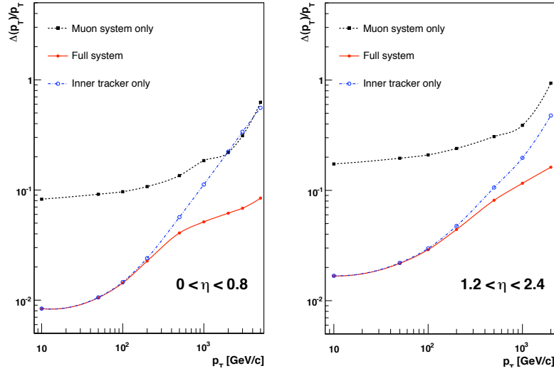
FIGURE 3.18: Muon momentum resolution as a function of p_T of muons in barrel and endcap regions.
