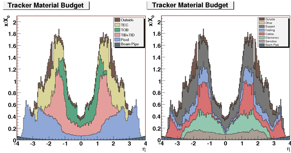
FIGURE 3.9: Material in radiation length's for different sub-detectors (left) and for different functional modules (right) as function of \eta [42].
