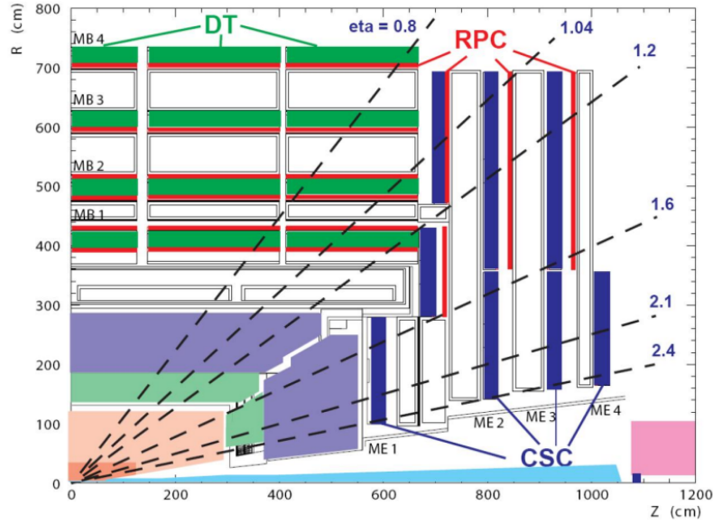
FIGURE 3.15: CMS muon system layout.
