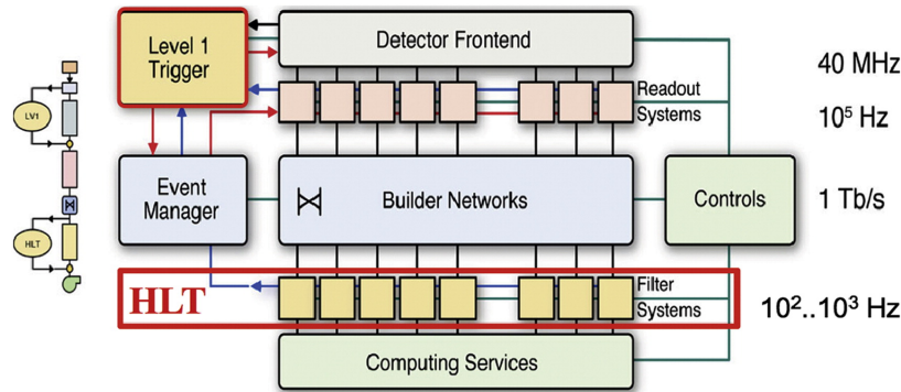
FIGURE 3.20: The CMS DAQ system structure.
