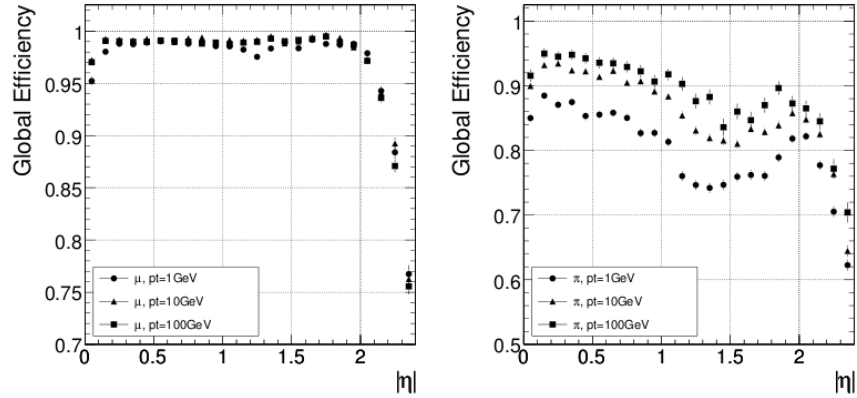
FIGURE 3.11: CMS tracker global efficiency of muons (left) and pions (right) of p_T = 1, 10, 100 GeV [42].
