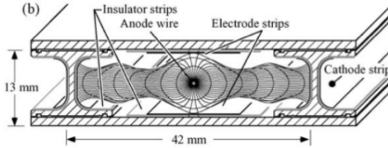
FIGURE 3.16: DT electric field created by cathode, anode and insulating strips .
