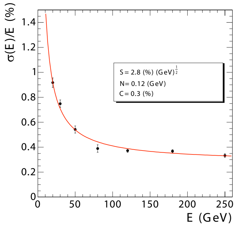
FIGURE 3.13: CMS ECAL expected energy resolution [42].
