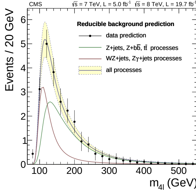
FIGURE 5.2: Prediction for the reducible background in all three channels together (black dots) fitted using an empirical shape (blue curve) with indicated total uncertainty (yellow band). Contributions from the 2P2F-like (green) and 3P1F-like (red) processes are fitted separately.
