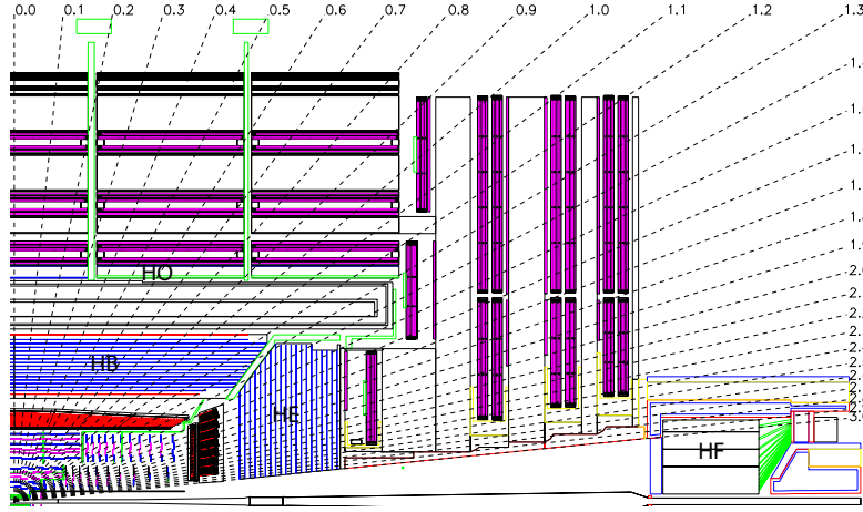
FIGURE 3.14: CMS HCAL layout.
