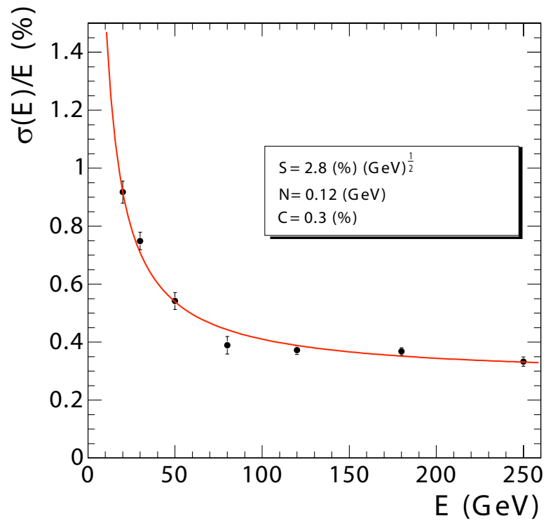
FIGURE 3.13: CMS ECAL expected energy resolution.
