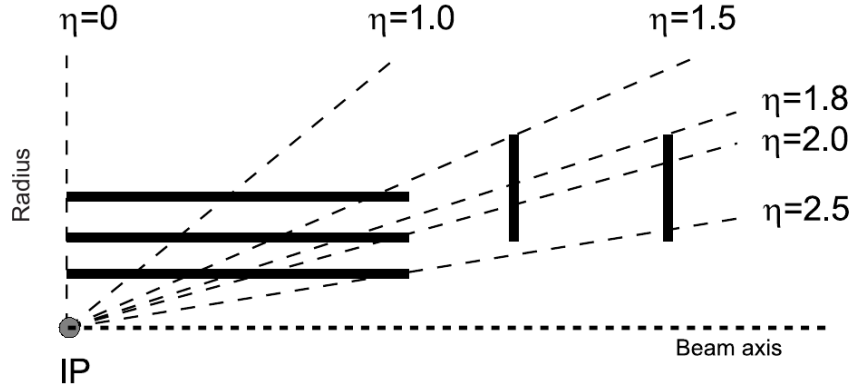
FIGURE 3.8: CMS pixel detectors and hit coverage. Lines represent detector modules.
