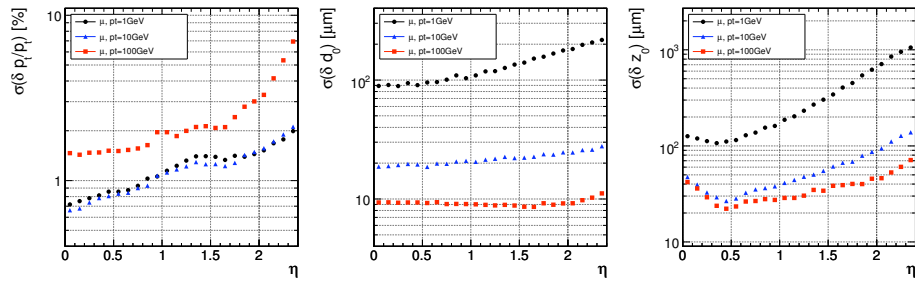
FIGURE 3.10: Expected single muons tracks resolution of transverse momentum (left), transverse impact parameter (middle) and longitudinal impact parameter (right) of p_T = 1, 10, 100 GeV.
