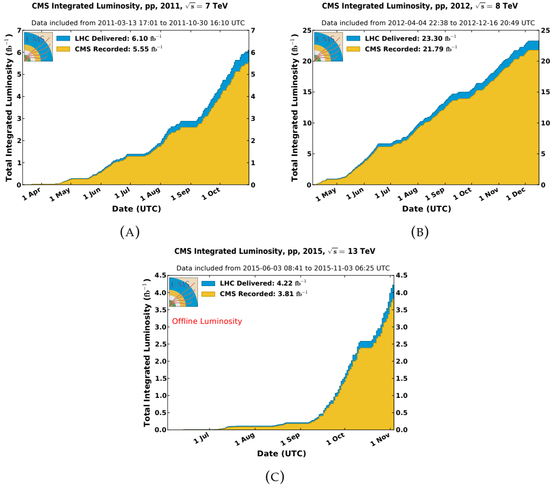
FIGURE 3.4: Integrated luminosities of LHC delivered (blue) and CMS recorded (yellow) data for 2011(a), 2012(b) and 2015(c)
