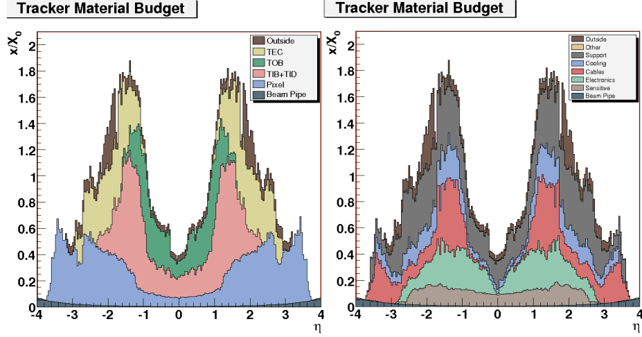
FIGURE 3.9: Material in radiation length's for different subdetectors (left) and for different functional modules (right) as function of \eta
