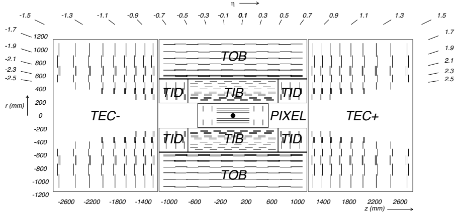
FIGURE 3.7: Schematic diagram of CMS tracker system. Lines represent detector modules.
