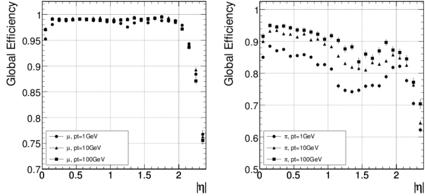
FIGURE 3.11: CMS tracker global efficiency of muons (left) and pions (right) of p_T = 1, 10, 100 GeV.
