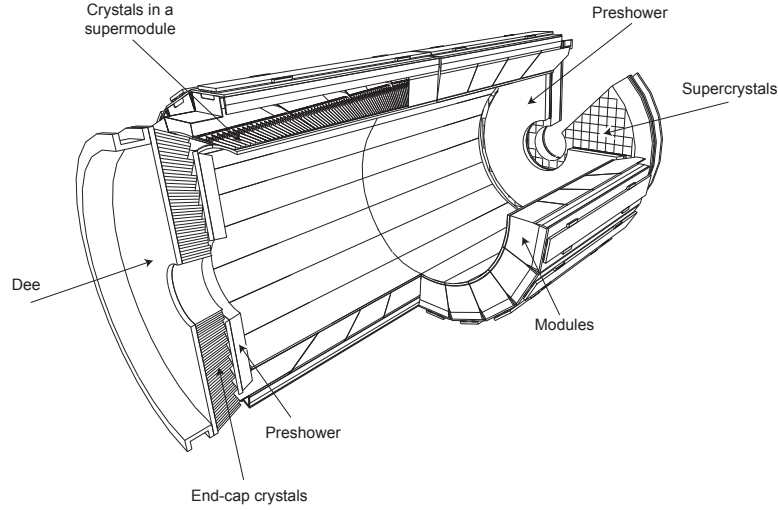
FIGURE 4.8: CMS ECAL layout
