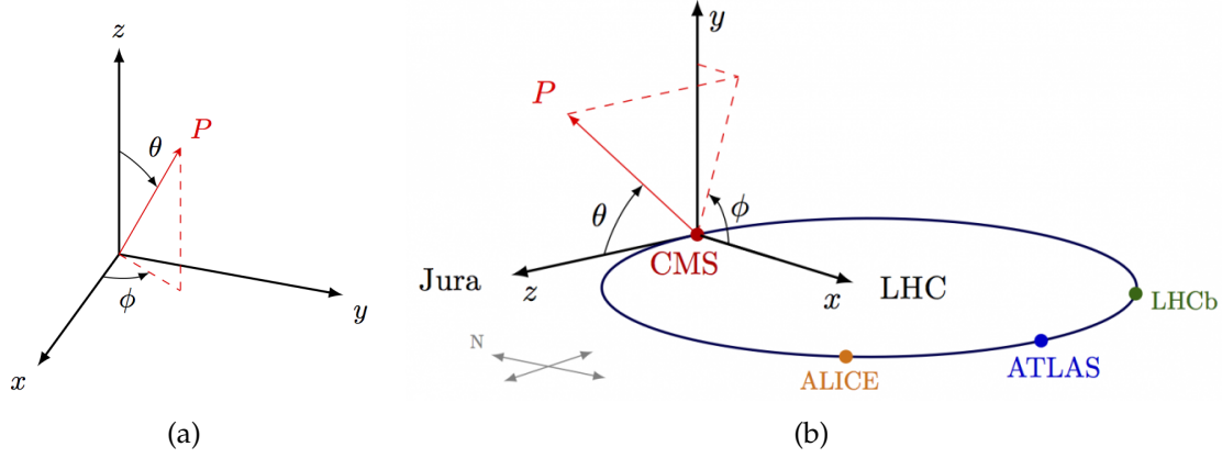
FIGURE 4.3: CMS spherical coordinte system
