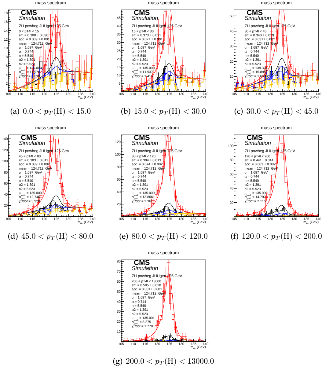
FIGURE 8.10: Example signal shapes at reconstruction level for a resonance of m(4\ell) in 4e final state for the ZH production mode from POWHEG+JHUGEN in different bins of p_T(H) . The black curve represents events which do not pass the fiducial volume selection. The curve has no effect on the result.
