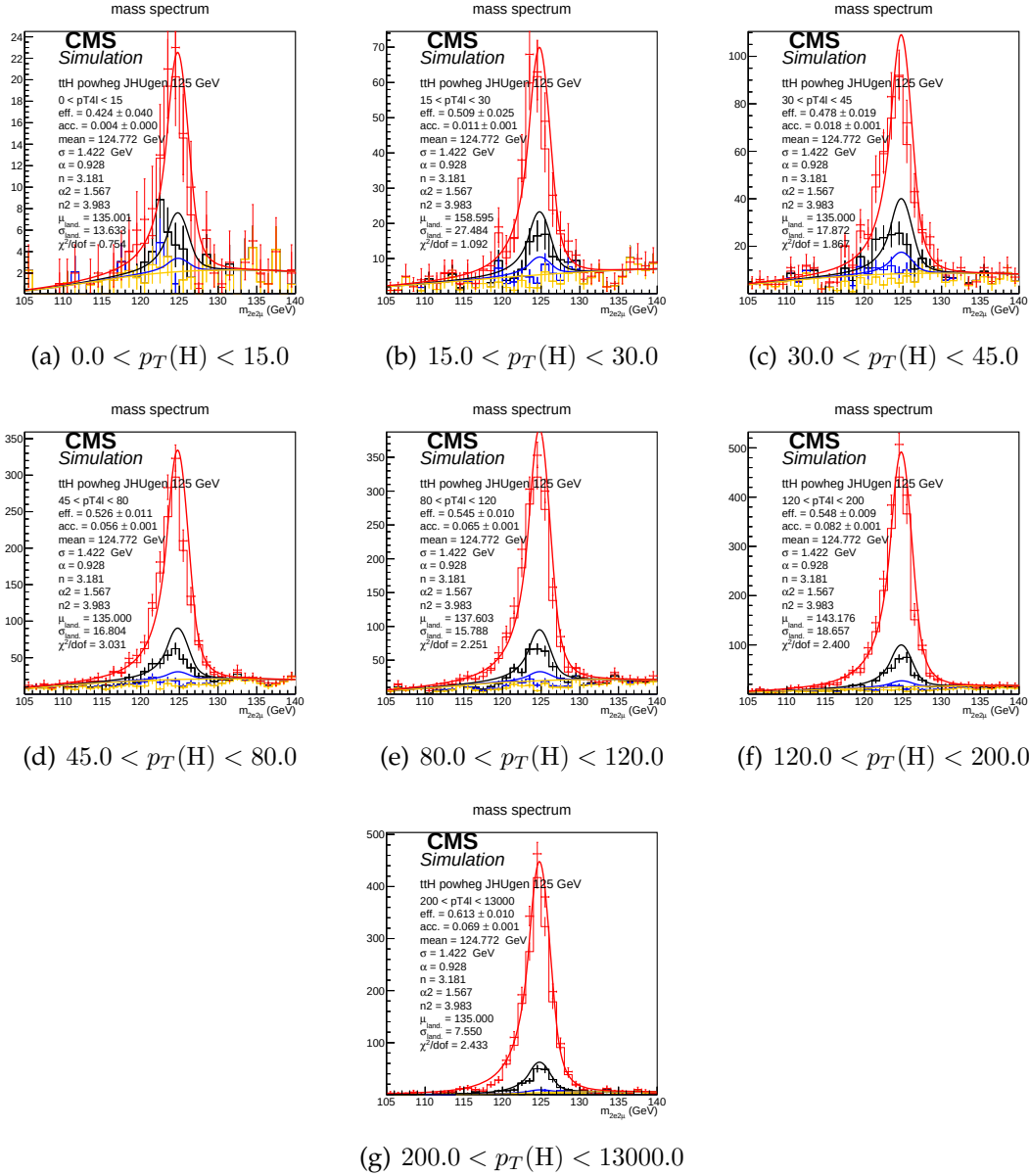
FIGURE 8.12: Example signal shapes at reconstruction level for a resonance of m(4\ell) in 2e2\mu final state for the ttH production mode from POWHEG+JHUGEN in different bins of p_T(H) . The black curve represents events which do not pass the fiducial volume selection. The curve has no effect on the result.
