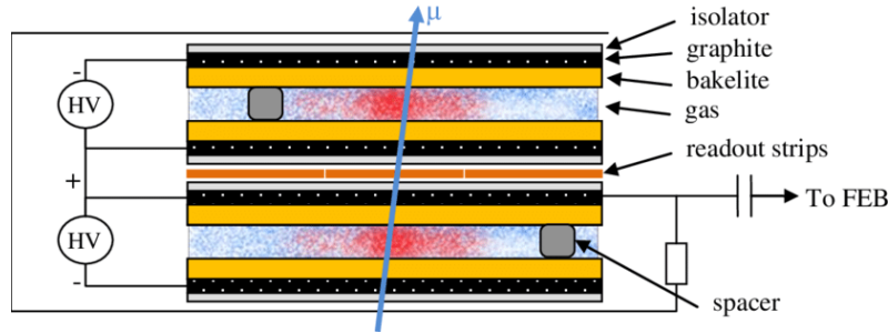
FIGURE 4.14: Cross sectional view of a RPC chamber.
