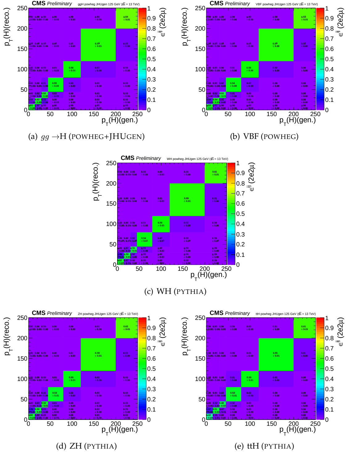
FIGURE 8.17: Efficiency matrices for p_T(H) for different SM production modes in the 2e2\mu final state.
