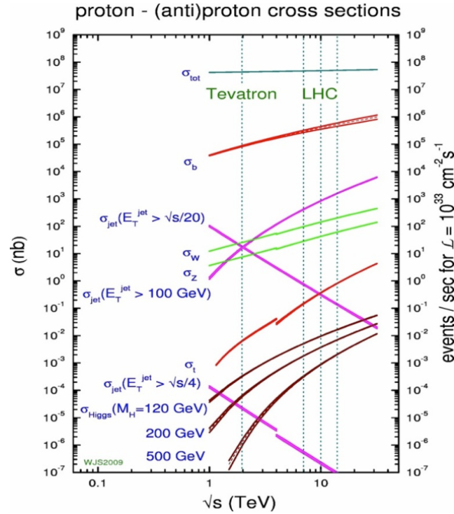
FIGURE 3.3: Cross section values for different processes corresponding to machine luminosity \mathcal{L} = 10^{33} \text{ cm}^2 \text{ s}^{-1} .
