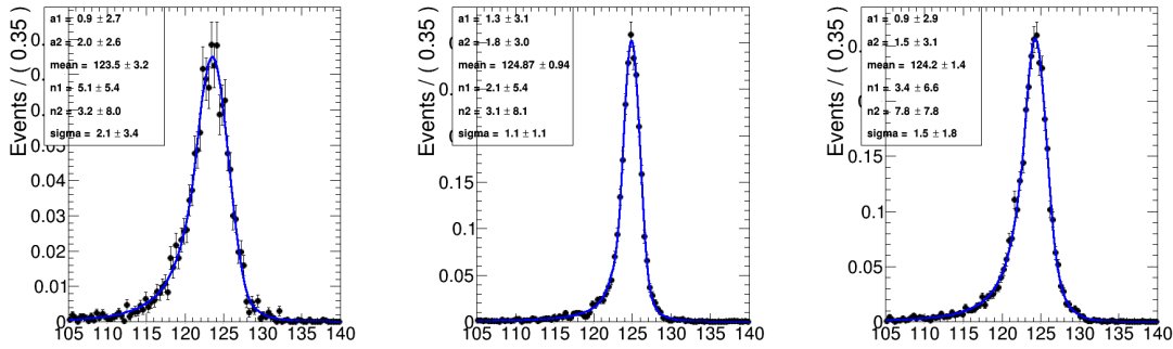
FIGURE 6.7: Probability density functions f(m_{4l}|m_H) for signal with m_H=125 GeV at the reconstruction level after the full lepton and event selections are applied. The distributions obtained from 13 TeV ggH MC samples are fitted with the model described in the text for 4\mu (left), 4e (center) and 2e2\mu (right) events. The distribution show the events for p_T below 10 GeV.
