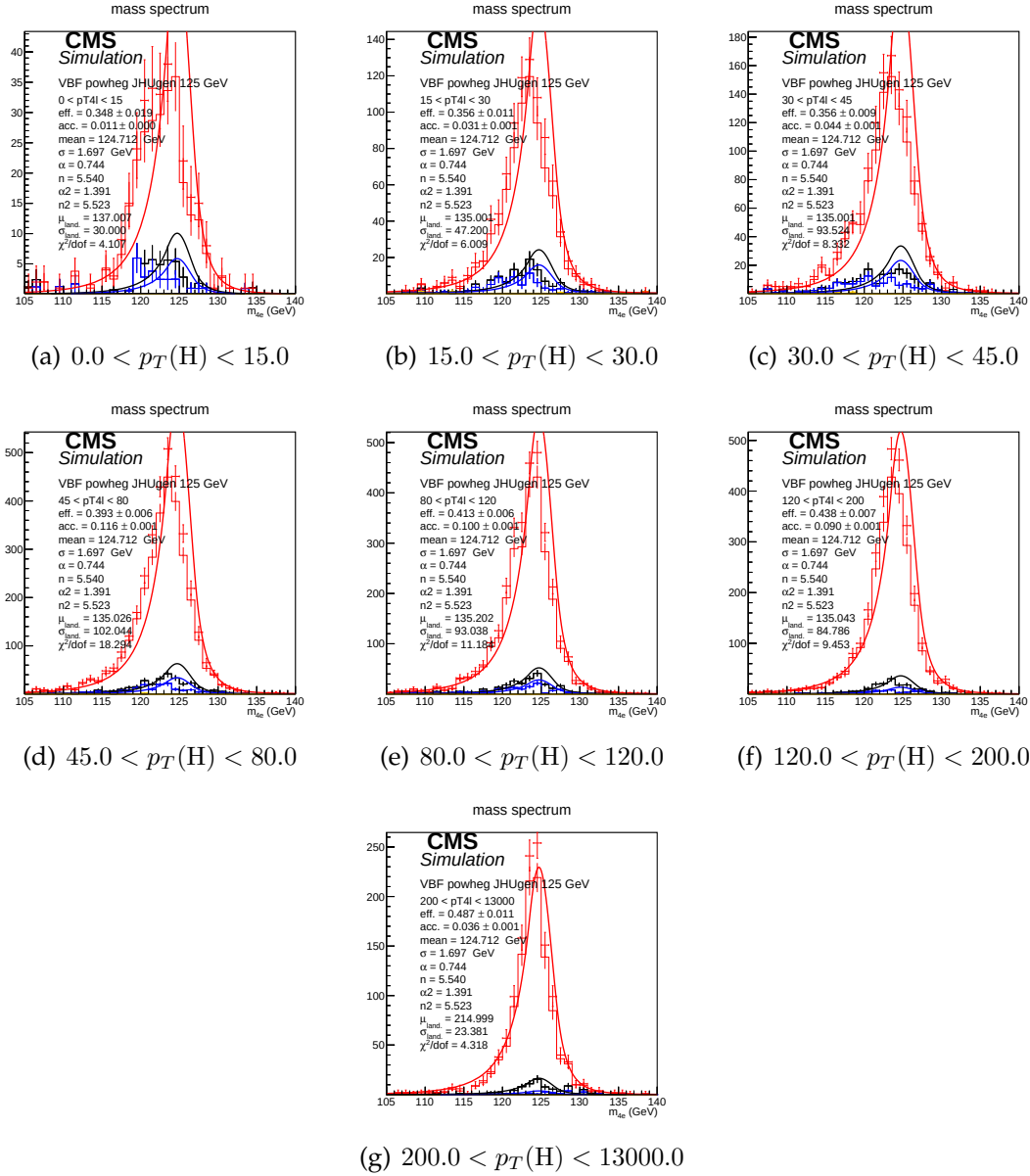
FIGURE 8.4: Example signal shapes at reconstruction level for a resonance of m(4\ell) in 4e final state for the VBF production mode from POWHEG+JHUGEN in different bins of p_T(H) . The black curve represents events which do not pass the fiducial volume selection. The curve has no effect on the result.
