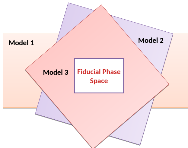
FIGURE 6.1: Fiducial phase definition among different models.
