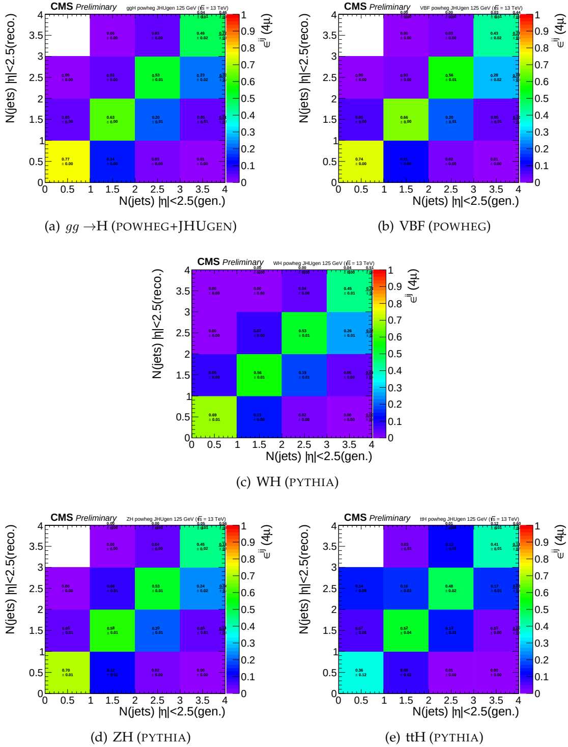
FIGURE 8.22: Efficiency matrices for N(\text{jets}) for different SM production modes in the 4\mu final state.
