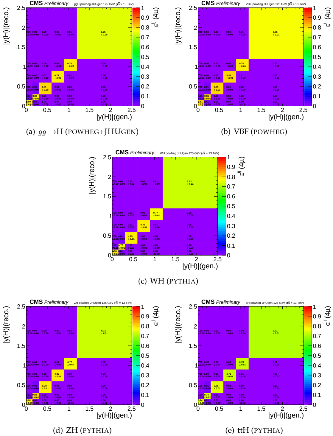
FIGURE 8.19: Efficiency matrices for |y(H)| for different SM production modes in the 4\mu final state.
