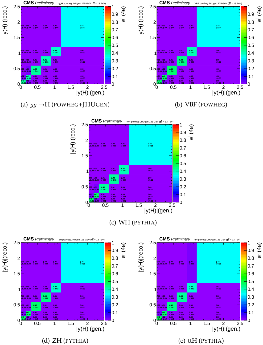
FIGURE 8.18: Efficiency matrices for |y(H)| for different SM production modes in the 4e final state.
