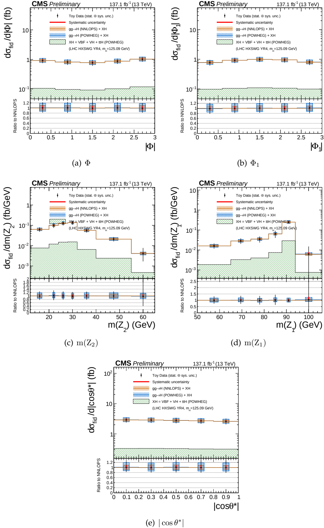
FIGURE 8.24: Differential fiducial cross section results using full Run 2 toy data for \Phi , \Phi_1 , m(Z_1) , m(Z_2) and |\cos \theta^*| in H \rightarrow 4\ell and comparison with the theoretical predictions.
