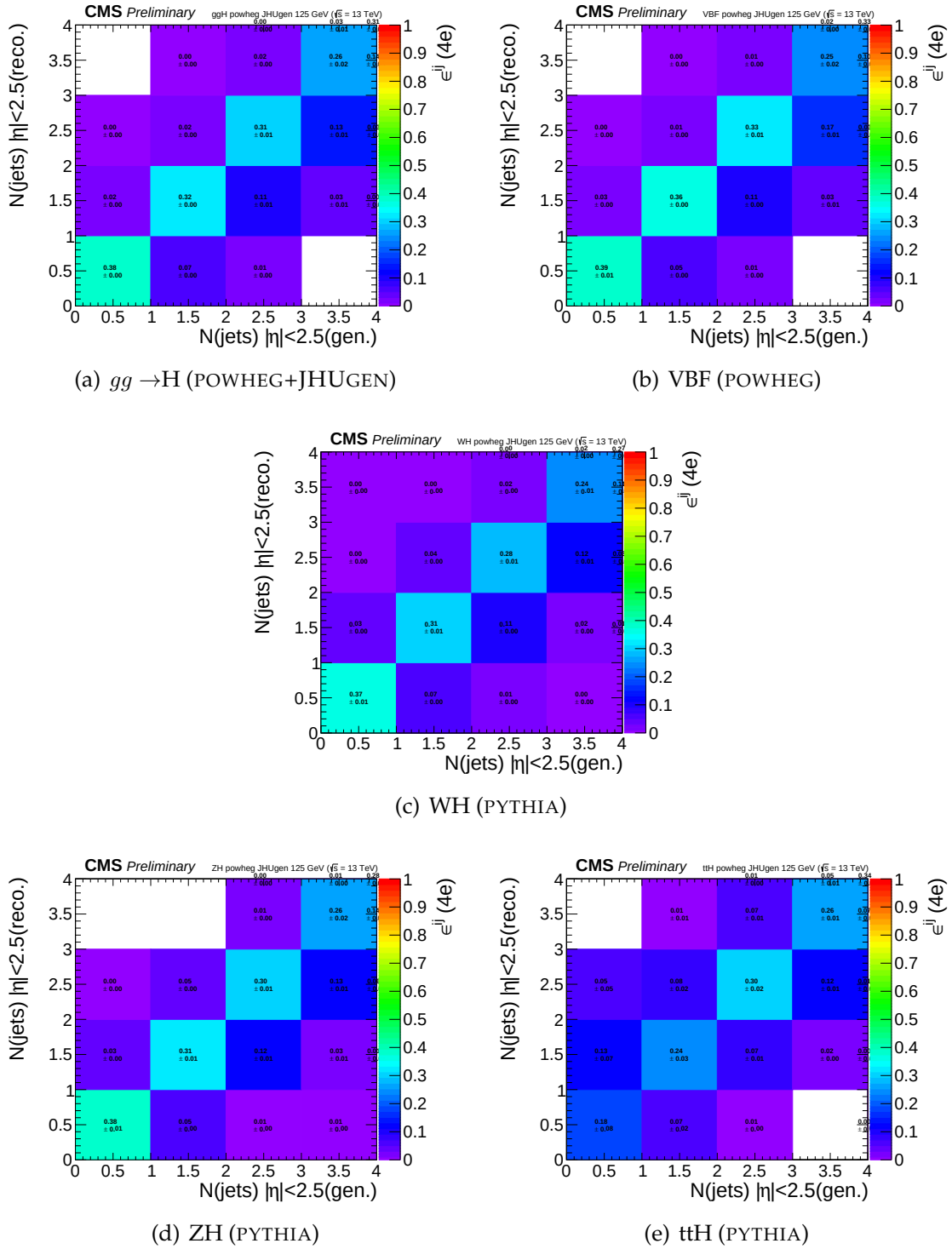
FIGURE 8.21: Efficiency matrices for N(\text{jets}) for different SM production modes in the 4e final state.
