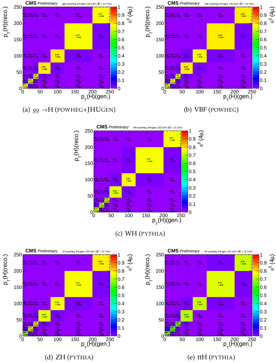
FIGURE 8.16: Efficiency matrices for p_T(H) for different SM production modes in the 4\mu final state.
