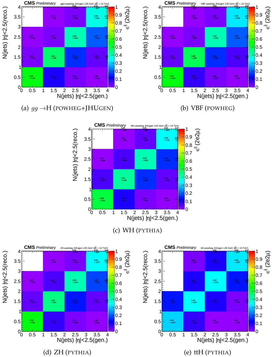
FIGURE 8.23: Efficiency matrices for N(\text{jets}) for different SM production modes in the 2e2\mu final state.
