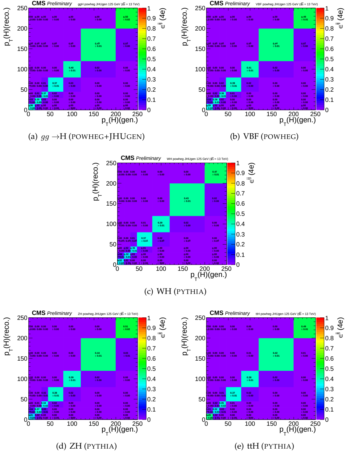
FIGURE 8.15: Efficiency matrices for p_T(H) for different SM production modes in the 4e final state.
