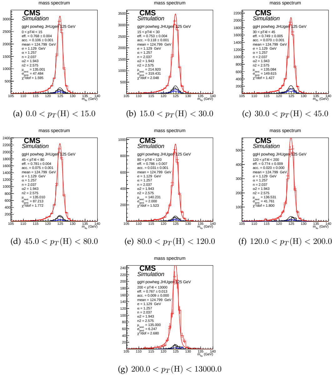
FIGURE 8.2: Example signal shapes at reconstruction level for a resonance of m(4\ell) in 4\mu final state for the gg \rightarrow H production mode from POWHEG+JHUGEN in different bins of p_T(H) . The black curve represents events which do not pass the fiducial volume selection. The curve has no effect on the result.
