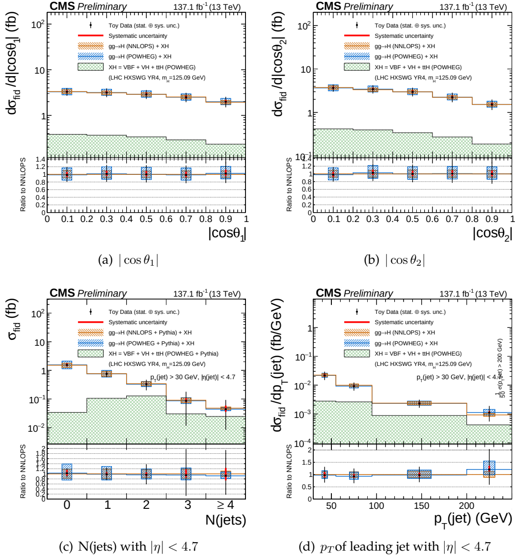
FIGURE 8.25: Differential fiducial cross section results using full Run 2 toy data for |\cos \theta_1| , |\cos \theta_2| , number of jets (within |\eta| < 4.7 ) and p_T of leading jet (within |\eta| < 4.7 ) in H \rightarrow 4\ell and comparison with the theoretical predictions. Systematic uncertainty is indicated by red bars and black bars show total statistical and the systematic uncertainties, combined in quadrature. The blue and brown colors show the theoretical predictions. The acceptances and the theoretical uncertainties in differential bins are computed using POWHEG. Sub-dominant production contributions XH = \text{VBF} + \text{VH} + t\bar{t}H are shown in green separately. The systematic uncertainties correspond to the generators accuracy are also taken in to account for differential predictions. The fraction of 4\mu , 4e and 2e2\mu in each differential bin is allowed to float in fit.
