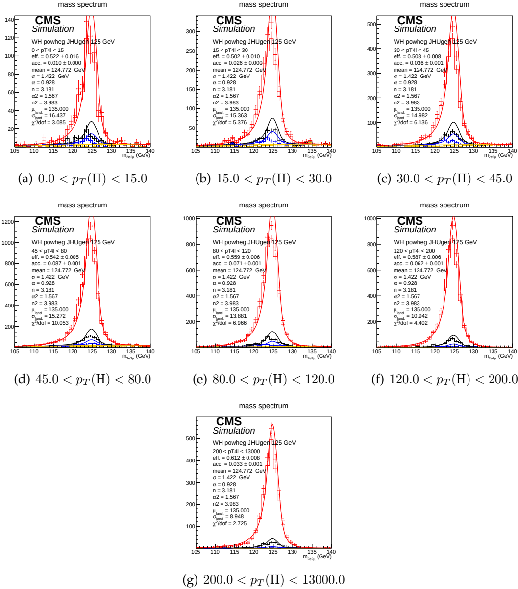
FIGURE 8.6: Example signal shapes at reconstruction level for a resonance of m(4\ell) in 2e2\mu final state for the WH production mode from POWHEG+JHUGEN in different bins of p_T(H) . The black curve represents events which do not pass the fiducial volume selection. The curve has no effect on the result.
