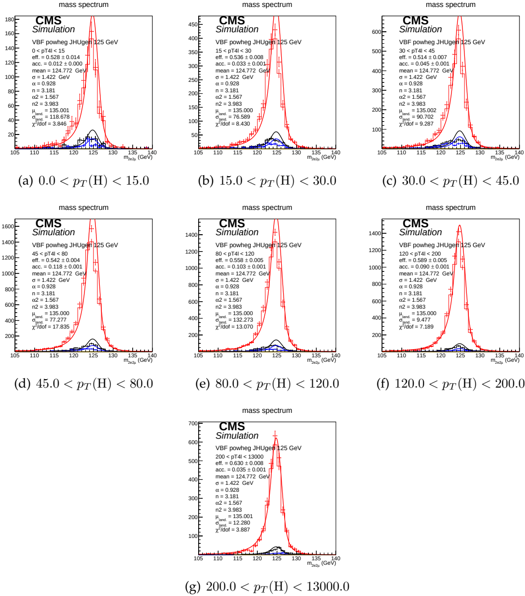
FIGURE 8.3: Example signal shapes at reconstruction level for a resonance of m(4\ell) in 2e2\mu final state for the VBF production mode from POWHEG+JHUGEN in different bins of p_T(H) . The black curve represents events which do not pass the fiducial volume selection. The curve has no effect on the result.
