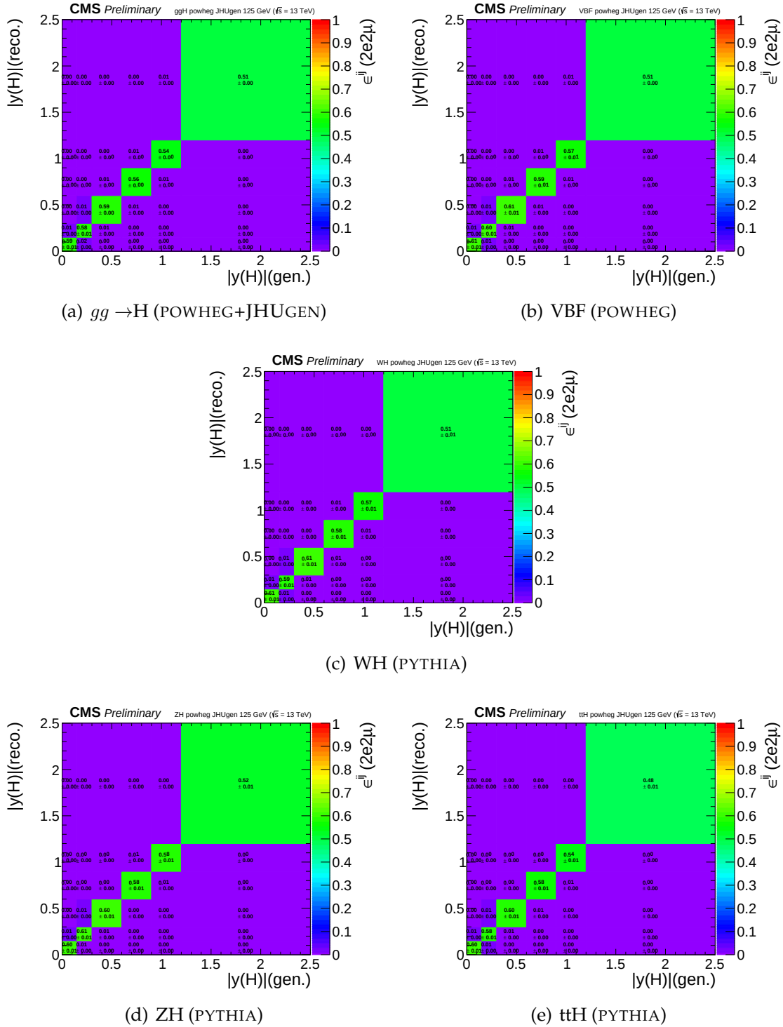
FIGURE 8.20: Efficiency matrices for |y(H)| for different SM production modes in the 2e2\mu final state.
