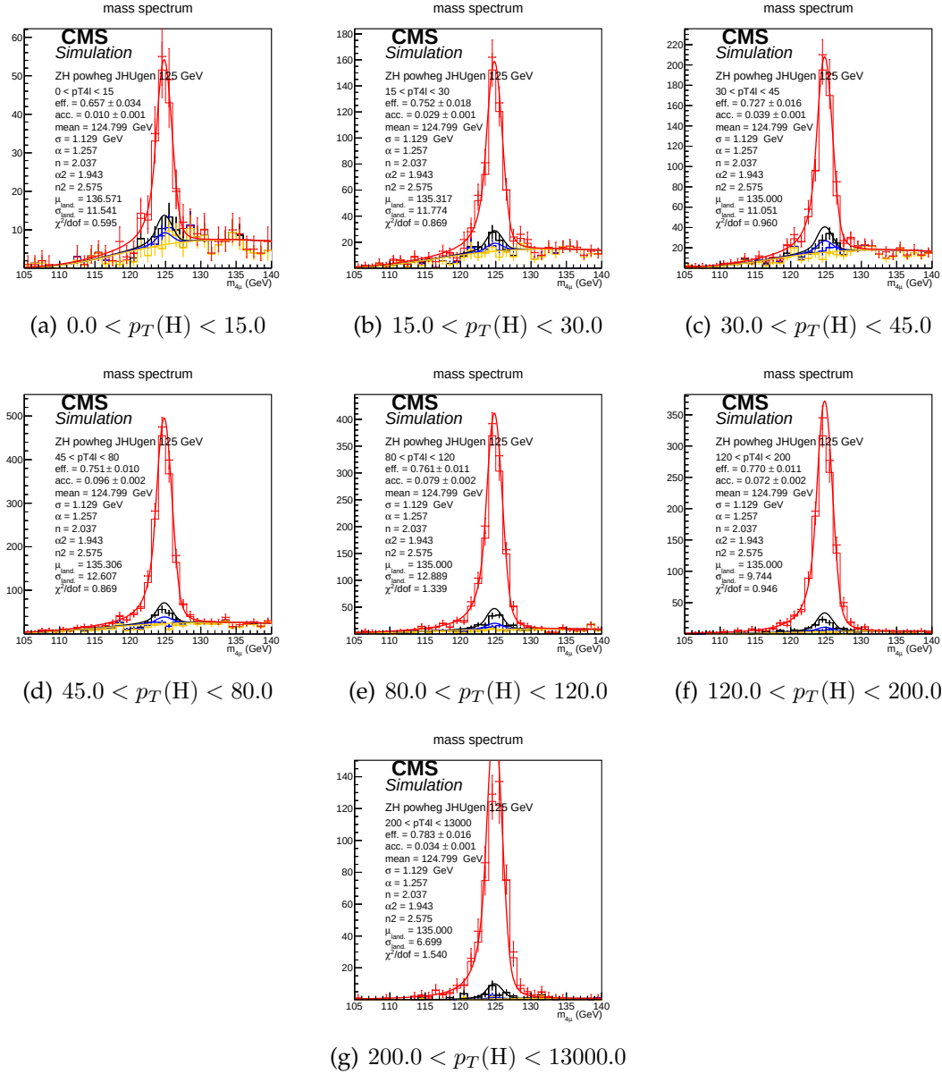
FIGURE 8.11: Example signal shapes at reconstruction level for a resonance of m(4\ell) in 4\mu final state for the ZH production mode from POWHEG+JHUGEN in different bins of p_T(H) . The black curve represents events which do not pass the fiducial volume selection. The curve has no effect on the result.
