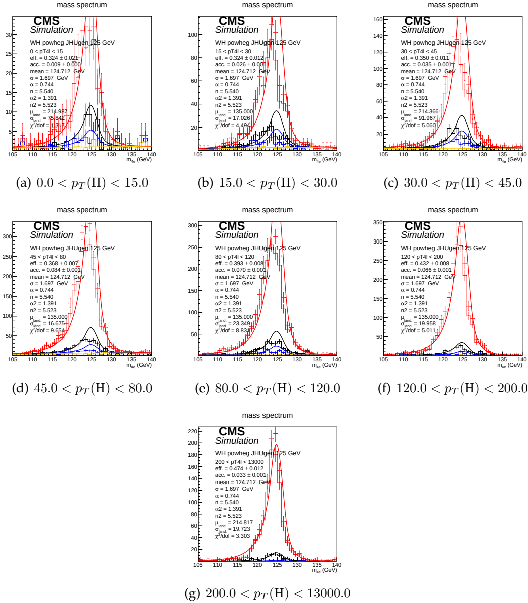
FIGURE 8.7: Example signal shapes at reconstruction level for a resonance of m(4\ell) in 4e final state for the WH production mode from POWHEG+JHUGEN in different bins of p_T(H) . The black curve represents events which do not pass the fiducial volume selection. The curve has no effect on the result.
