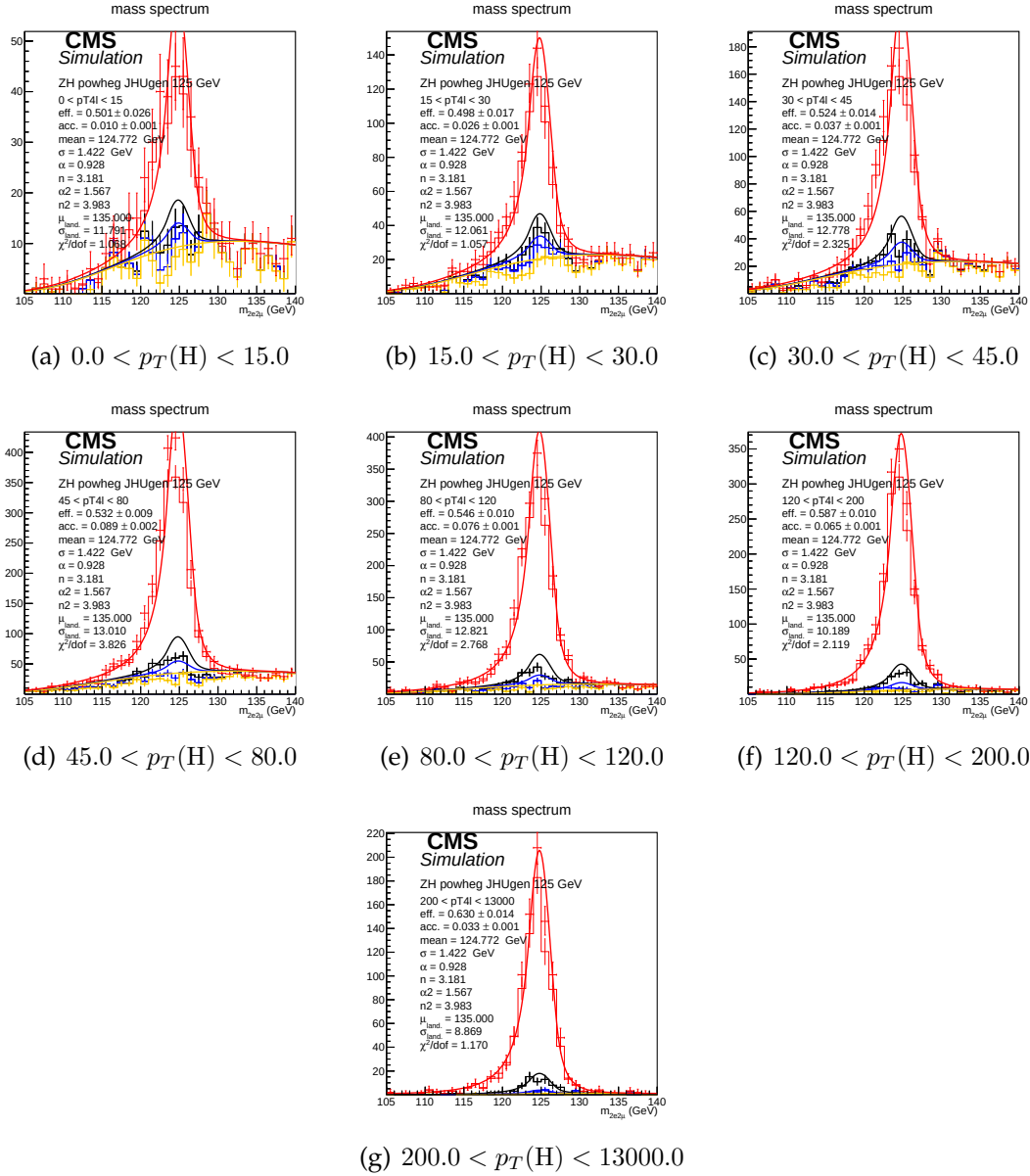
FIGURE 8.9: Example signal shapes at reconstruction level for a resonance of m(4\ell) in 2e2\mu final state for the ZH production mode from POWHEG+JHUGEN in different bins of p_T(H) . The black curve represents events which do not pass the fiducial volume selection. The curve has no effect on the result.
