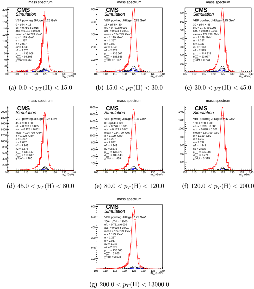
FIGURE 8.5: Example signal shapes at reconstruction level for a resonance of m(4\ell) in 4\mu final state for the VBF production mode from POWHEG+JHUGEN in different bins of p_T(H) . The black curve represents events which do not pass the fiducial volume selection. The curve has no effect on the result.
