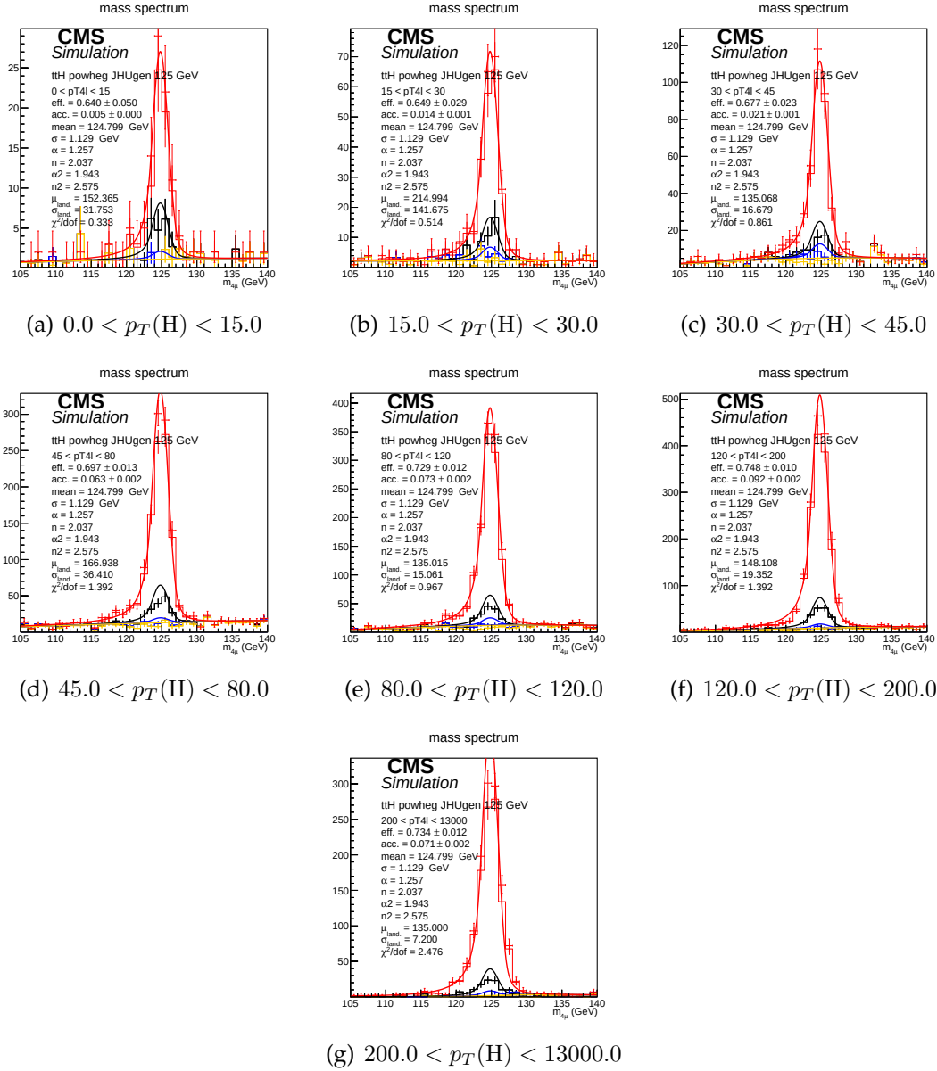
FIGURE 8.14: Example signal shapes at reconstruction level for a resonance of m(4\ell) in 4\mu final state for the ttH production mode from POWHEG+JHUGEN in different bins of p_T(H) . The black curve represents events which do not pass the fiducial volume selection. The curve has no effect on the result.
