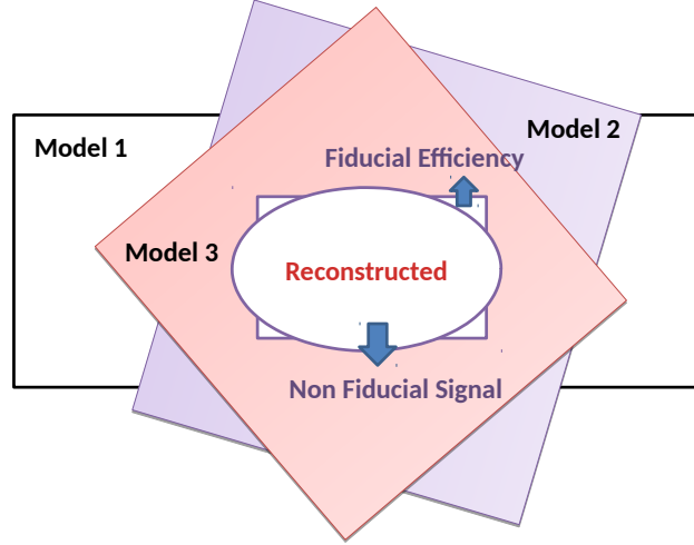
FIGURE 6.6: Fiducial efficiency( \epsilon ) and nonfiducial( f_{nonfid} ) signal definition.
