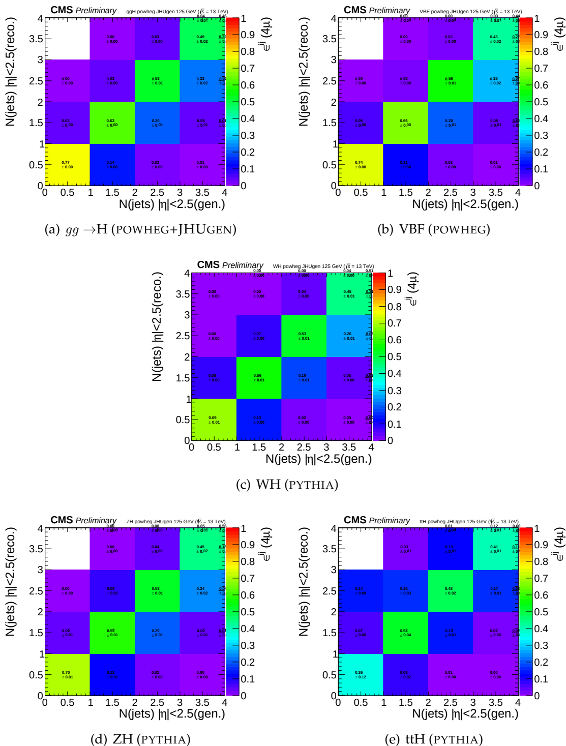
FIGURE 8.22: Efficiency matrices for N(\text{jets}) for different SM production modes in the 4\mu final state.
