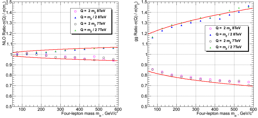
FIGURE 2: QCD scale uncertainties for (left) pp \rightarrow ZZ \rightarrow 4\ell at NLO and (right) gg \rightarrow ZZ \rightarrow 4\ell processes. The points are evaluated uncertainties. The curves are the fit systematic error \kappa(m_{4\ell}) to be used in the statistical analysis. These errors are driven by two independent nuisance parameters QCDscale\_VV for pp \rightarrow ZZ \rightarrow 4\ell at NLO and QCDscale\_ggVV for gg \rightarrow ZZ \rightarrow 4\ell .
