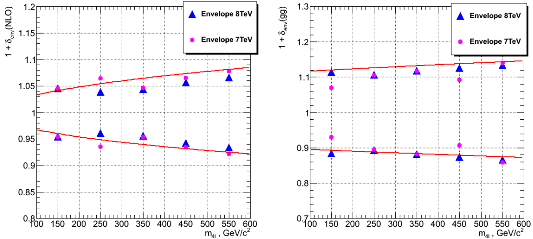
FIGURE 1: PDF+ \alpha_s uncertainties for (left) pp \rightarrow ZZ \rightarrow 4\ell at NLO and (right) gg \rightarrow ZZ \rightarrow 4\ell processes. The points are evaluated uncertainties. The curves are the fit systematic error \kappa(m_{4\ell}) to be used in the statistical analysis. These errors are driven by two independent nuisance parameters pdf\_qqbar for pp \rightarrow ZZ \rightarrow 4\ell at NLO and pdf\_gg for gg \rightarrow ZZ \rightarrow 4\ell .
