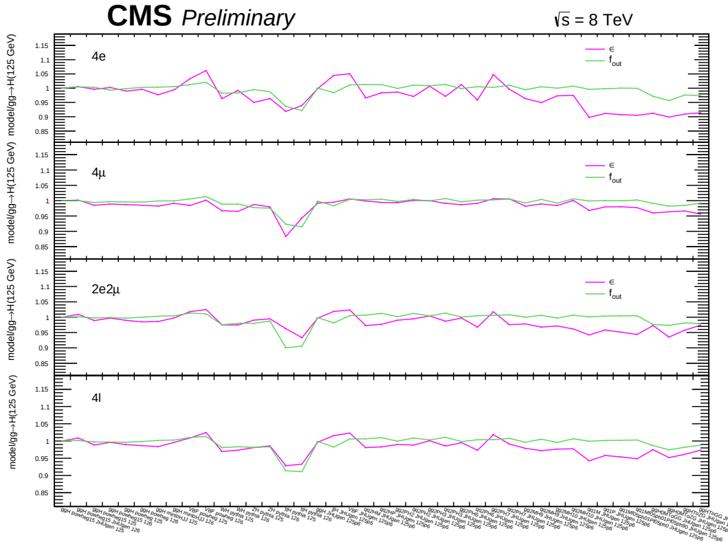
FIGURE 3: Ratio of integrated \epsilon and f_{\text{nonfid}} for all signal models to the integrated \epsilon and f_{\text{nonfid}} from the gg \rightarrow H production mode (POWHEG+JHUGEN 125 GeV).
