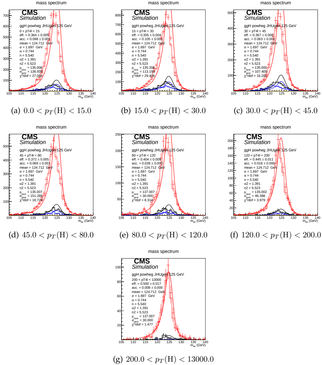
FIGURE 8.1: Example signal shapes at reconstruction level for a resonance of m(4\ell) in 4e final state for the gg \rightarrow H production mode from POWHEG+JHUGEN in different bins of p_T(H) . The black curve represents events which do not pass the fiducial volume selection. The curve has no effect on the result.
