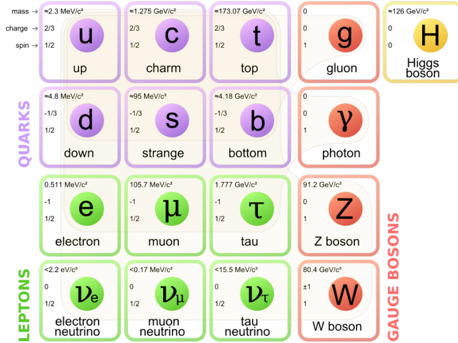
FIGURE 1.1: The elementary particles given in three generations of matter, the gauge bosons in fourth column and the Higgs boson in the fifth.
