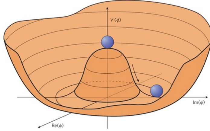
FIGURE 1.3: The Higgs potential as in Eq.1.6
