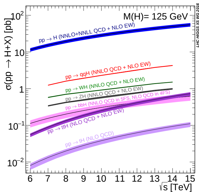
FIGURE 1.6: Production cross sections of Higgs boson ( m_H = 125 GeV) as a function of center of mass energies
