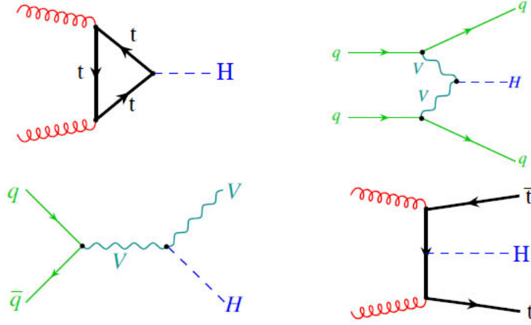
FIGURE 1.4: Feynman diagrams of Higgs production at tree level: gluon-gluon fusion (upper left); VV fusion (upper right); associated production with W and Z bosons (bottom left); associated production with t\bar{t} (bottom right).
