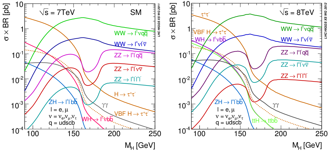
FIGURE 1.8: Cross sections of Higgs times branching ratios at 7 TeV and 8 TeV (left and right diagrams respectively).
