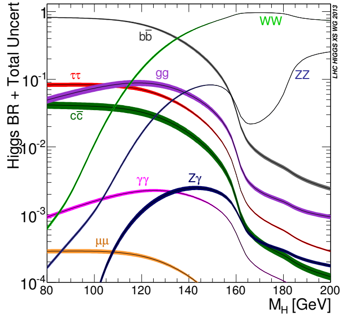
FIGURE 1.7: Branching ratios for different Higgs boson decay channels as a function of the Higgs mass.
