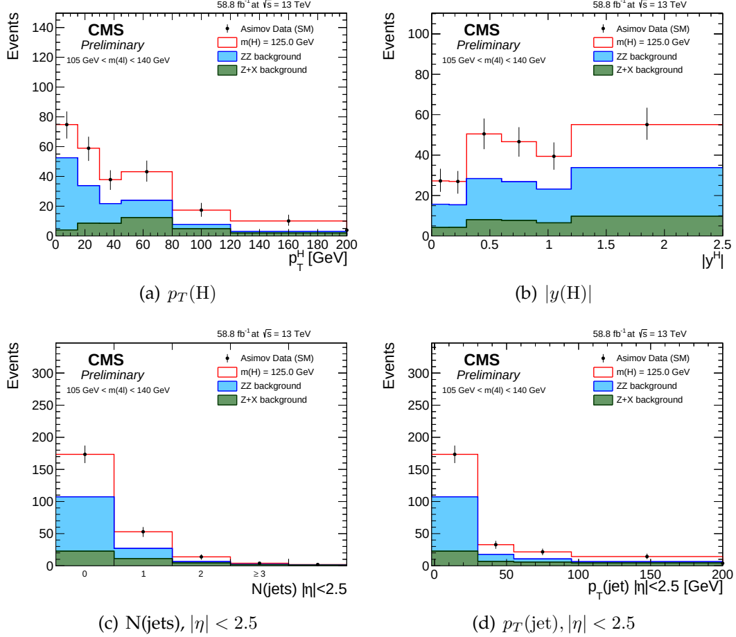
FIGURE 5.15: Expected yield using 2018 Asimov data along with SM signal ( m_H = 125.09 \text{ GeV} ) and background expectations for different observables and for all final states combined, in mass window 105 < m_{4\ell} < 140 \text{ GeV} which is used for H \rightarrow 4\ell measurements. The extraction of the signal is performed by exploiting the differences in the expected m_{4\ell} spectra of the signal and the background contributions in each differential bin of an observable.
