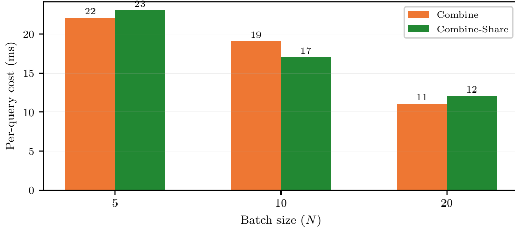
Figure 4: Per-query amortized cost vs. batch size. Both batched modes drop from about 22 ms to about 11 ms as batch size grows from 5 to 20.
