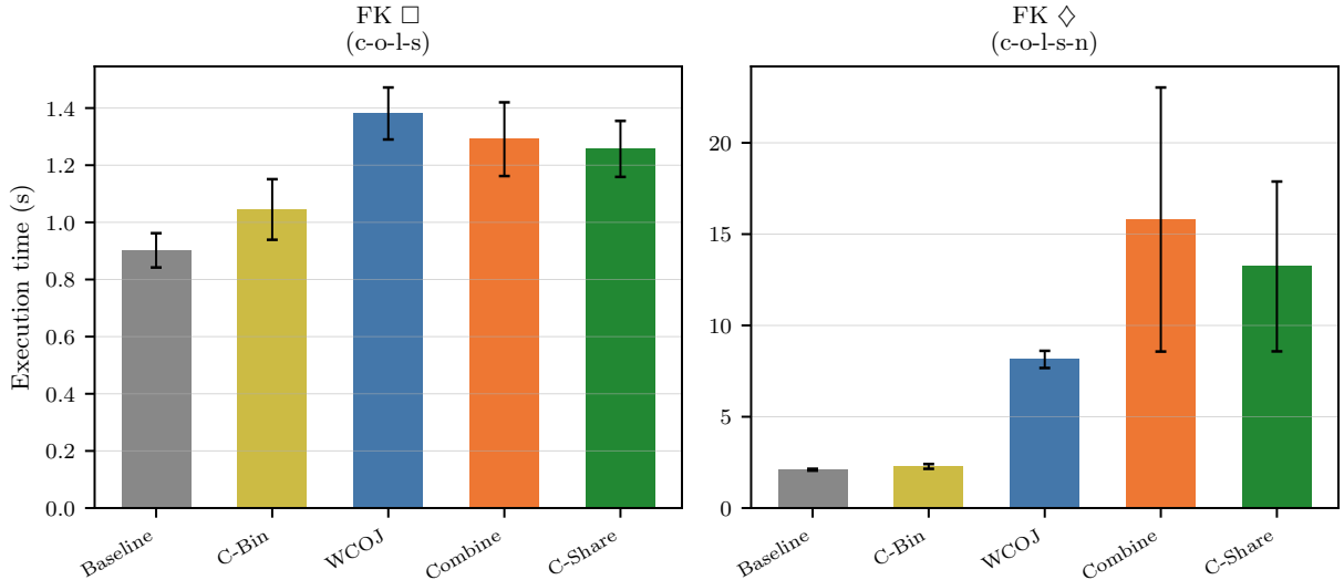
Figure 7: TPC-H FK cyclic performance. WCOJ regresses 1.5x on the rectangle and 3.9x on the diamond. Combine and Combine-Share compound the regression on the diamond due to materialization overhead.
