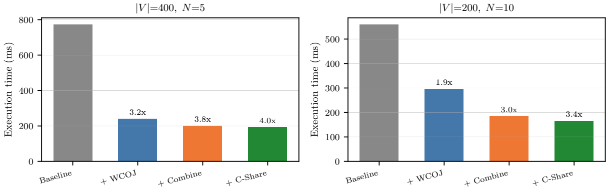
Figure 5: Optimization contributions waterfall at two operating points. WCOJ provides the dominant speedup; Combine and Combine-Share add incremental gains.
