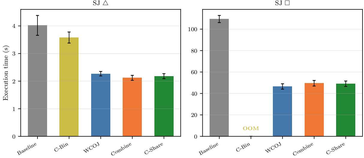
Figure 6: TPC-H self-join cyclic performance. WCOJ provides 1.8x speedup on the triangle and 2.4x on the 4-cycle. Binary joins OOM on the 4-cycle. Combine-binary (batching without WCOJ) contributes little on the triangle (1.1x).
