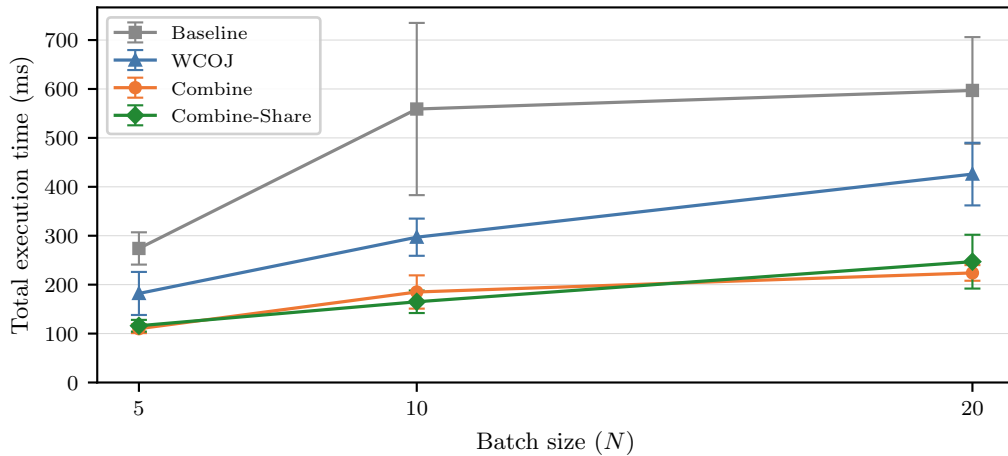
Figure 3: Total execution time vs. batch size. All modes scale sub-linearly; Combine-Share leads at N=10 but plain Combine overtakes at N=20 .
