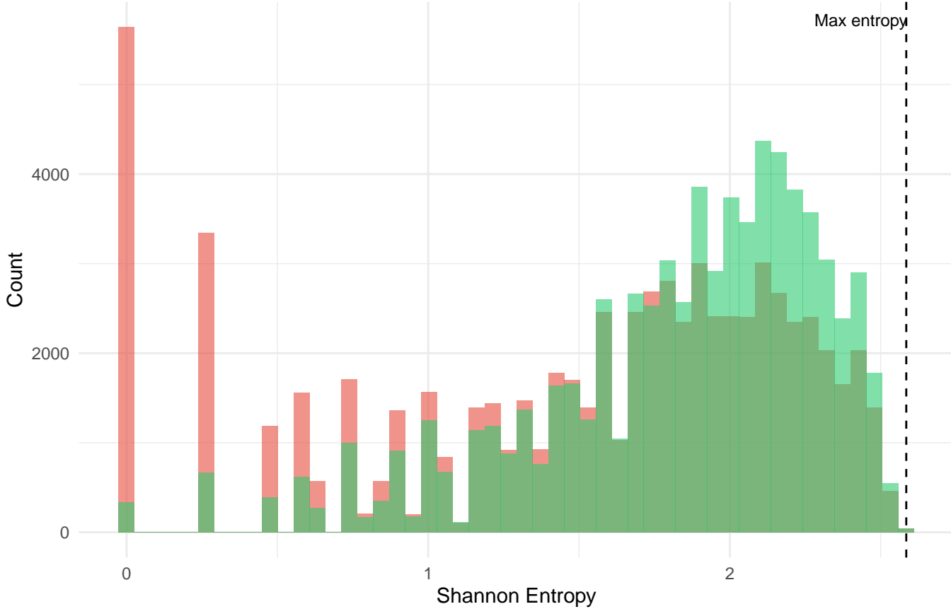
Per-Cell KNN Neighborhood Entropy Distribution
