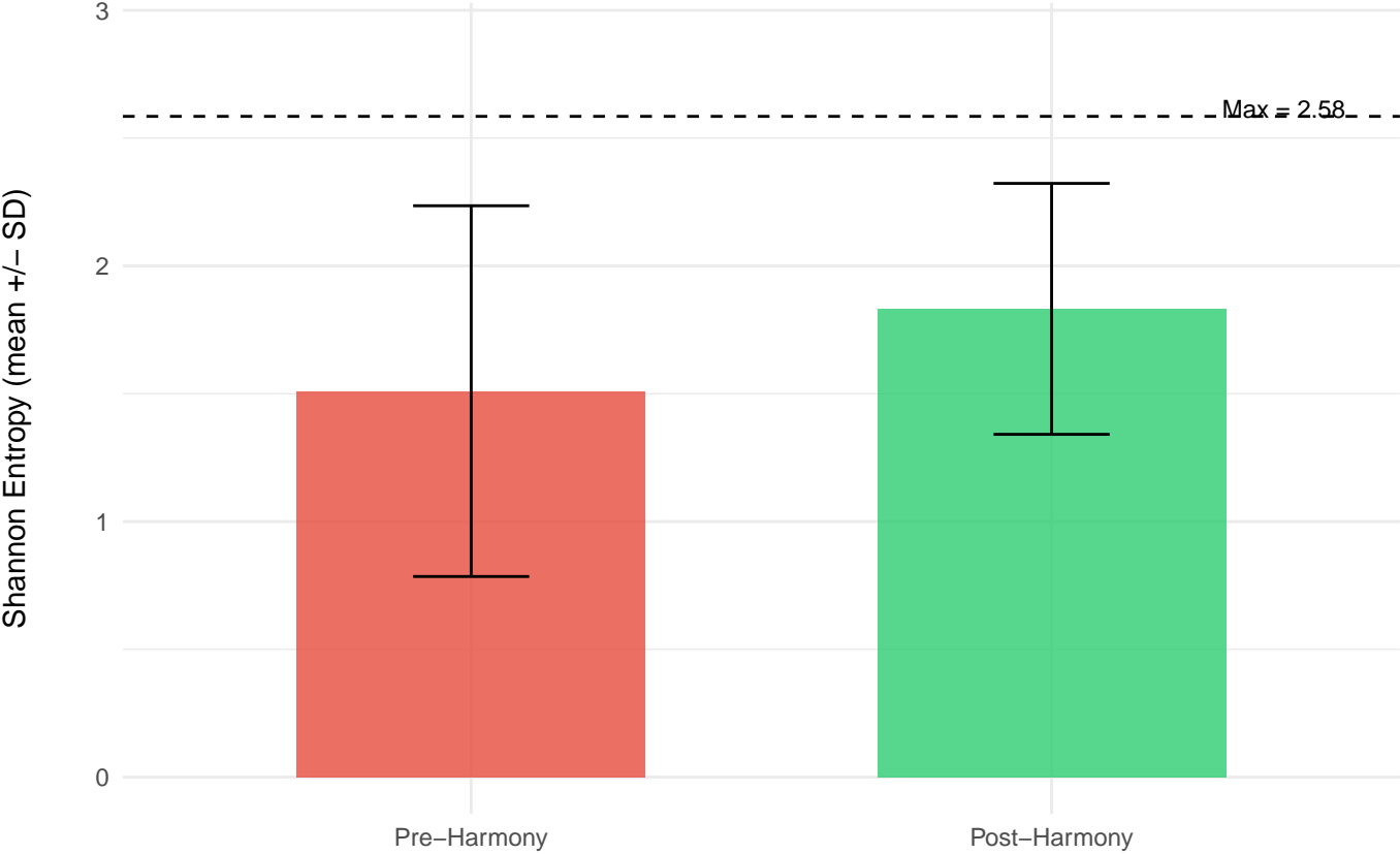
Mean Per-Cell KNN Entropy
