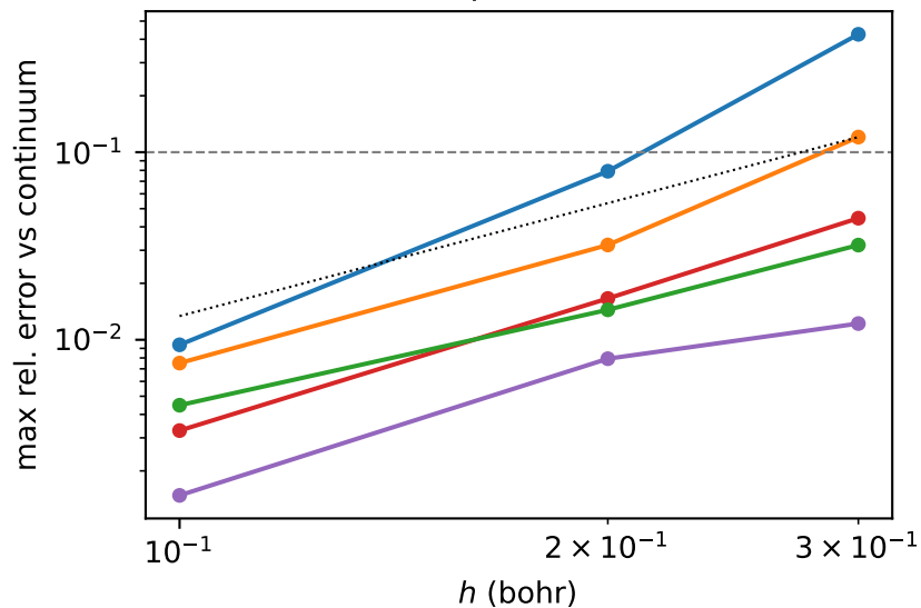
bispectrum
