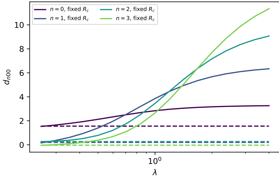
(a) d_{n00} under \rho \rightarrow \lambda^3 \rho(\lambda r) solid: R_c = 3 \text{ \AA} ; dashed: fixed \xi
