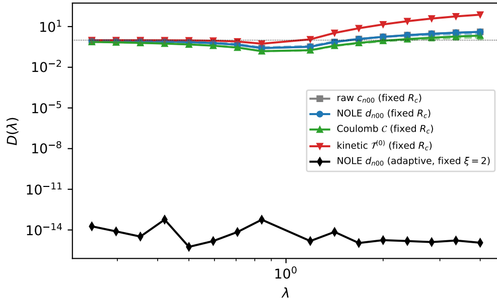
(b) relative deviation, R_c = 3 \text{ \AA} solid: hydrogenic; dashed: Gaussian
