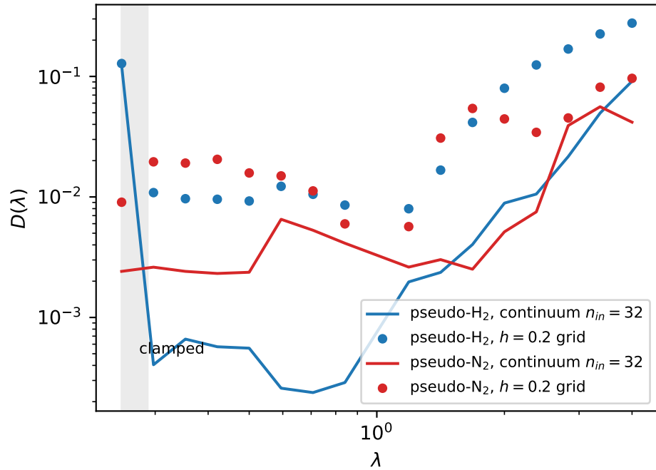
(b) scale invariance of the 3D pipeline (midpoint)
