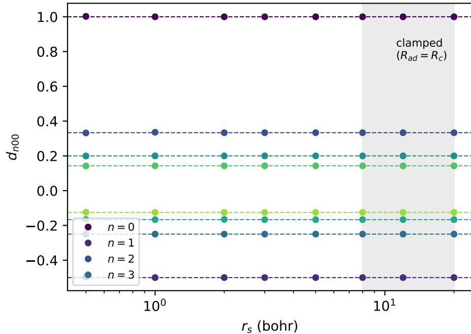
(a) HEG values on the h = 0.2 bohr grid
