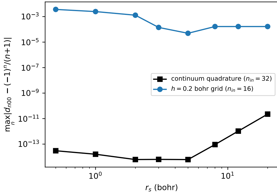
(b) deviation from the analytic HEG values
