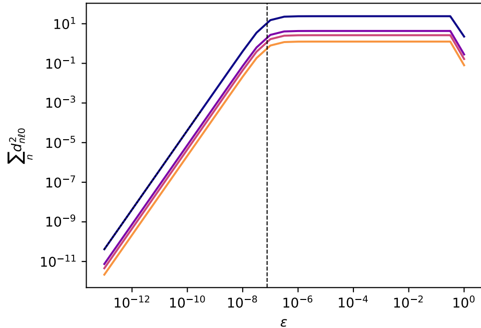
(b) power spectrum decay, \mathcal{O}(\varepsilon^2) guide
