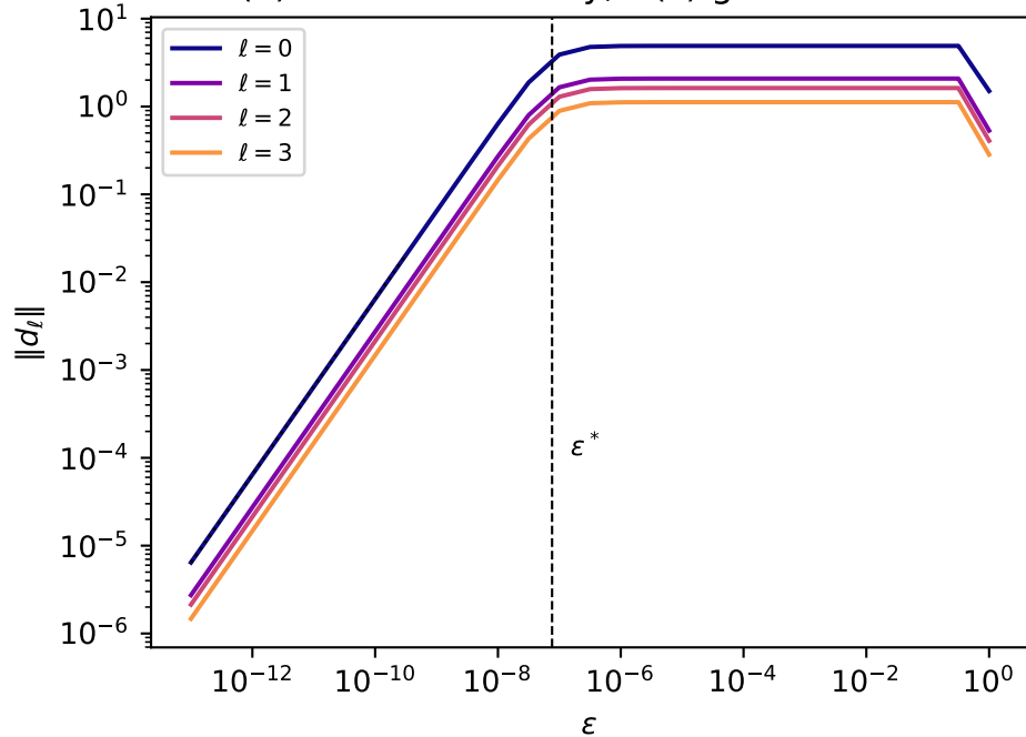
(a) coefficient decay, \mathcal{O}(\varepsilon) guide dotted
