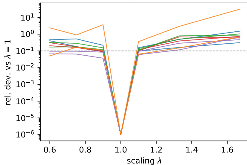
bispectrum
