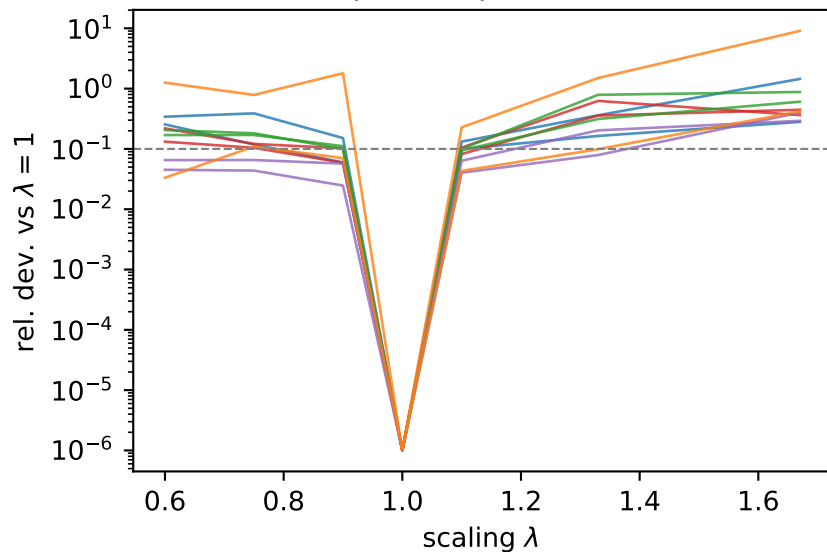
power spectrum
