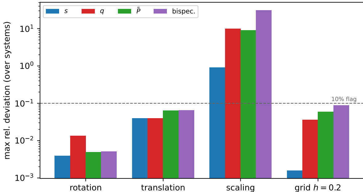
Invariance of SIMPLE features on 3D Cartesian grids ( R_c = 6 )
