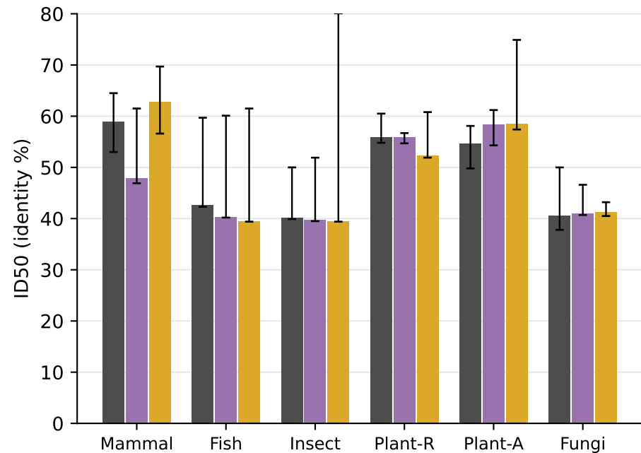
Fig 1B with 95% bootstrap CIs (1,000 resamples of the reference panel)
