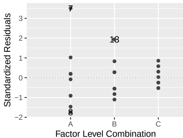
Constant Leverage: Residuals vs Factor Levels
