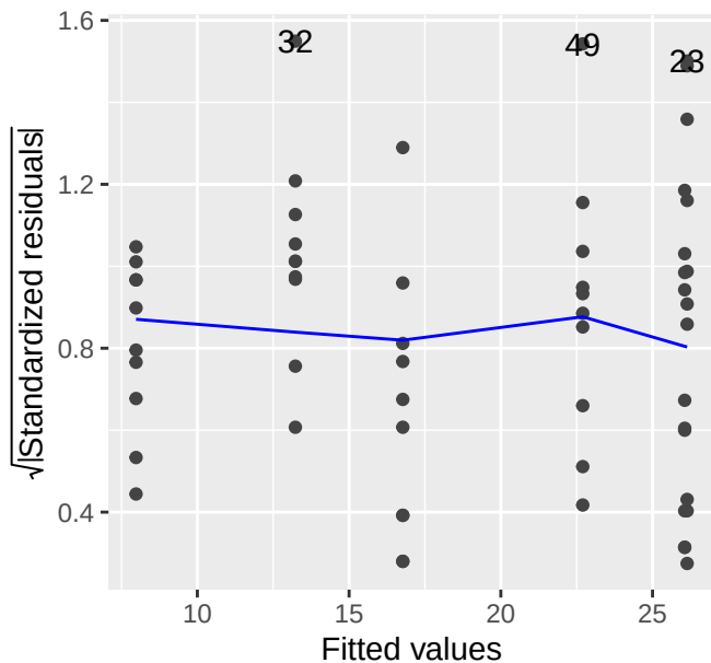
Scale-Location
