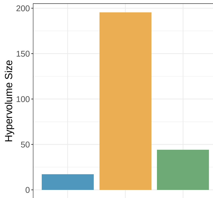
Total Hypervolumes
