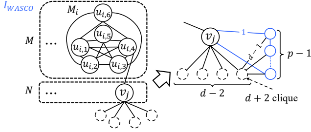
Figure 2: Gadget for the inapproximability reduction
