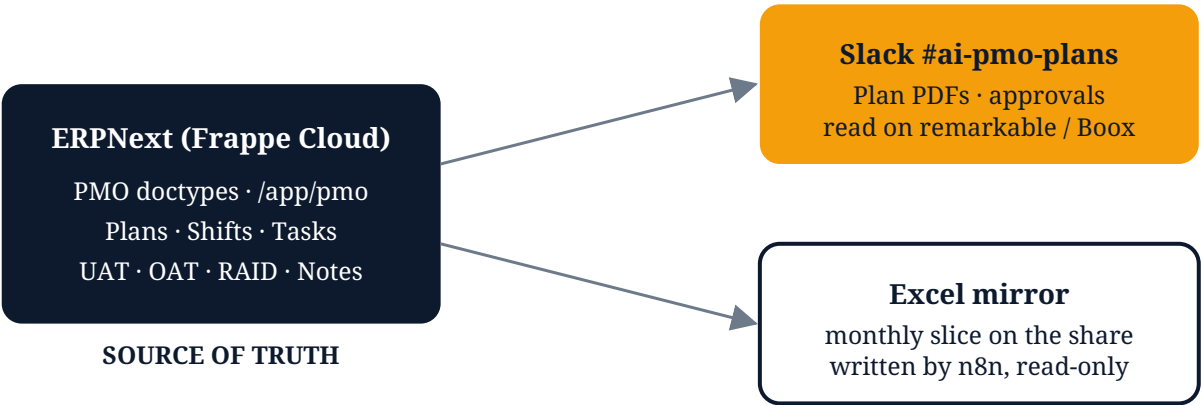
Figure 2. One source of truth, two downstream review surfaces. No reverse writes from Slack or Excel back into ERPNext.
