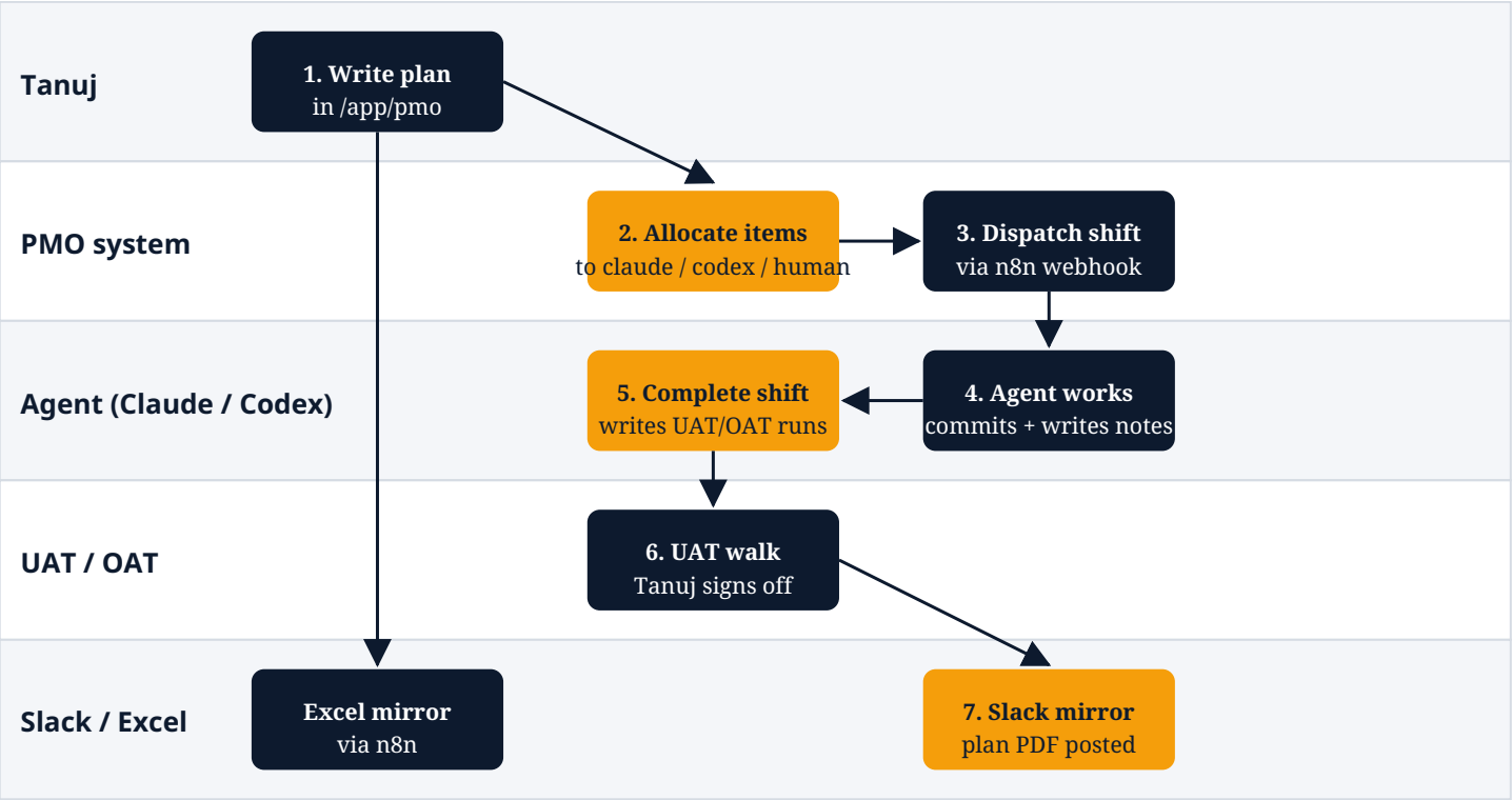
Figure 1. One full loop: from a plan in your head to tests signed off and notes mirrored to Slack and Excel.
