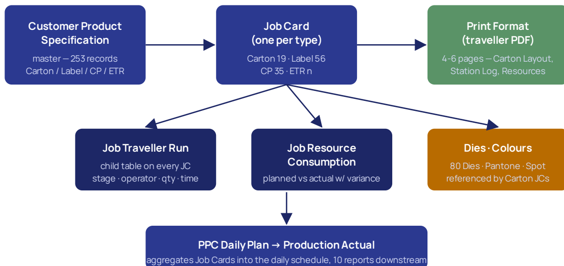
Figure 1. The CPS → Job Card → Print Format pipeline, with Traveller / Resource child tables feeding the PPC layer.
