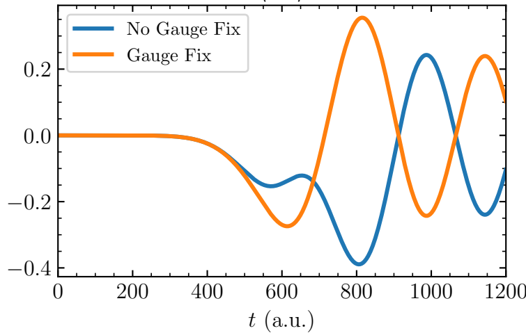
\langle \sigma_x \rangle
