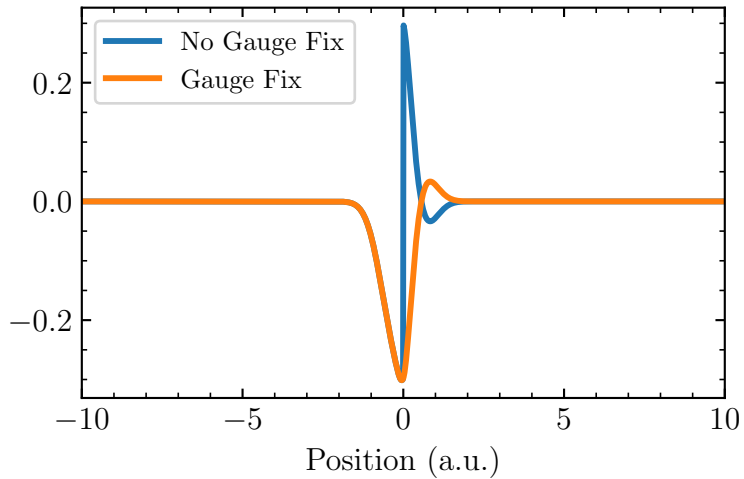
\sigma_x for t = 600 a.u.
