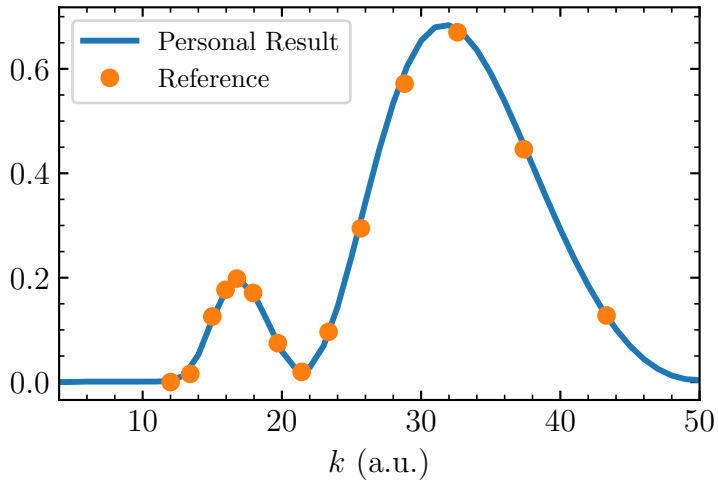
Dual Avoided Crossing
