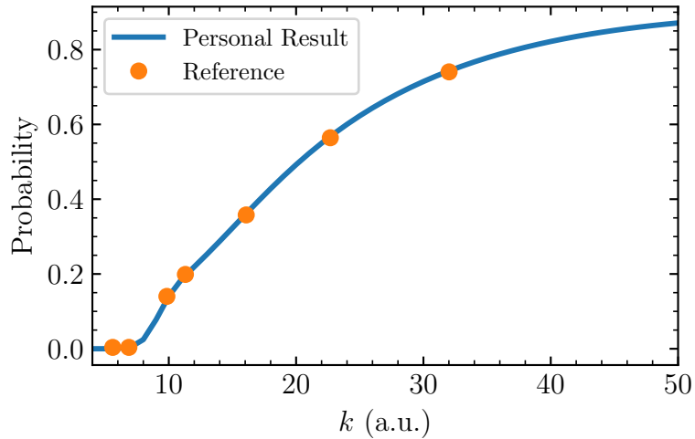
Single Avoided Crossing
