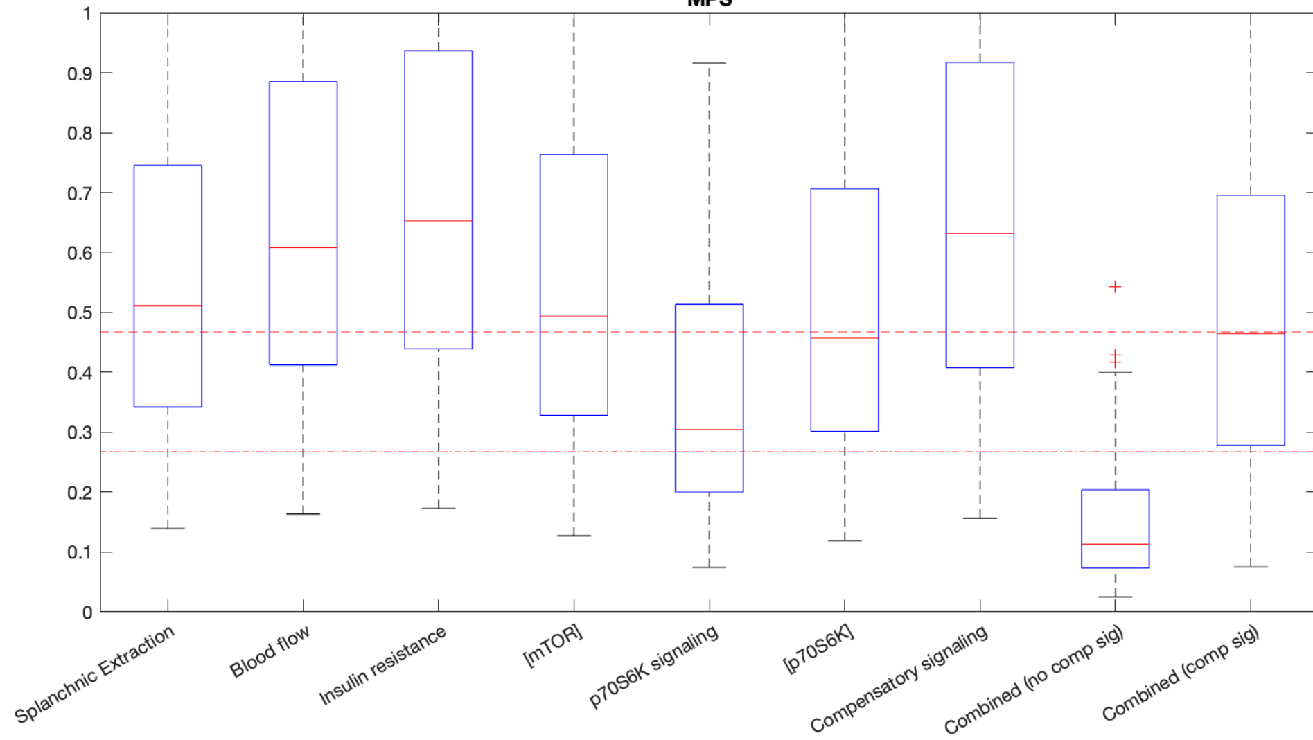
6: [p70S6K] MPS
