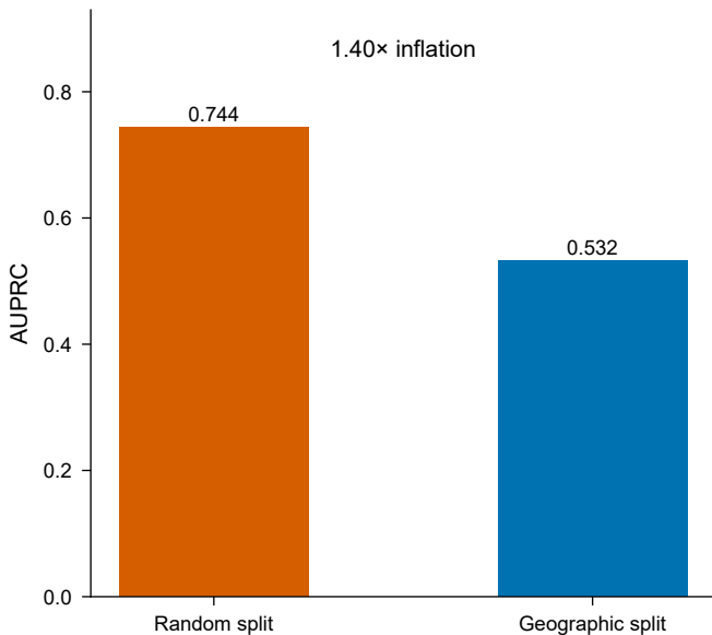
a Spatial leakage (evaluation protocol)
