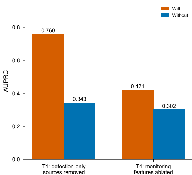
b Ascertainment (who is monitored)
