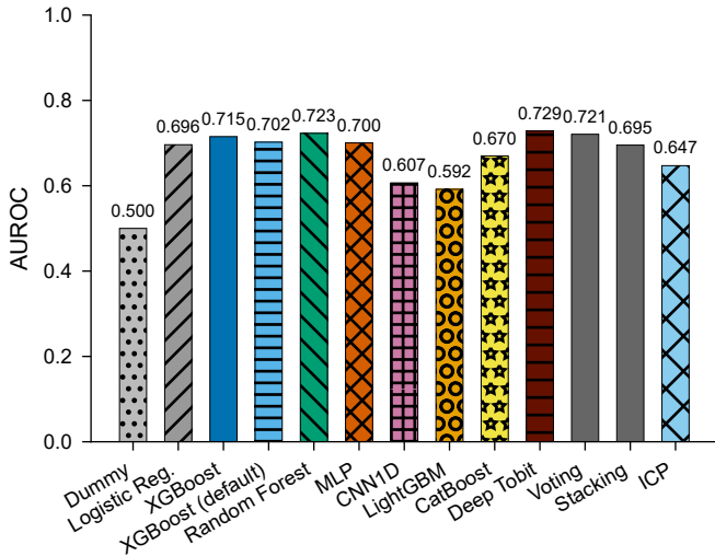
a T5 Transfer AUROC
