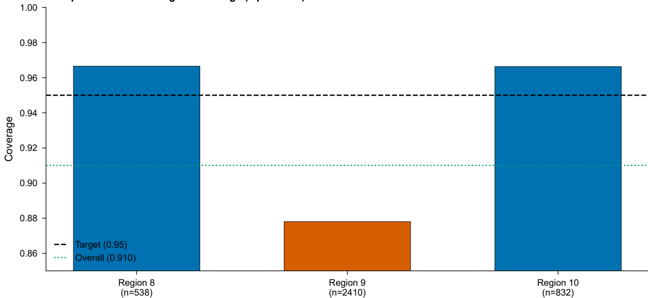
Group Conformal Per-Region Coverage (alpha=0.05)
