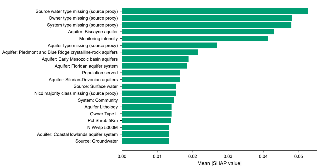
Feature Importance (T1 XGBoost)
