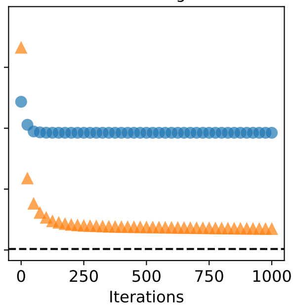
Error scaling: 1
