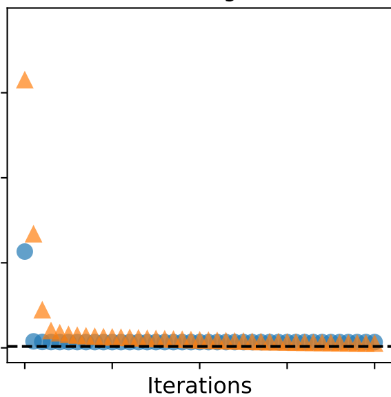
Error scaling: 0.01
