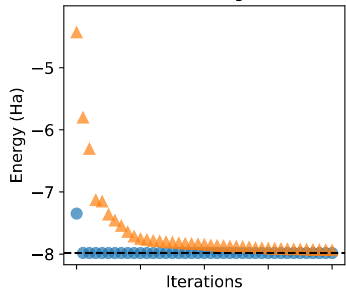
Error scaling: 0
