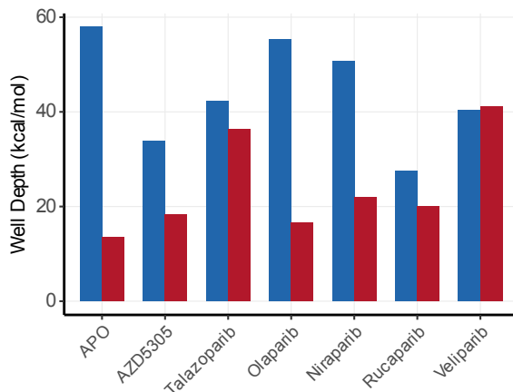
B HD-ART Energy Landscape: DNA-free vs DNA-bound
