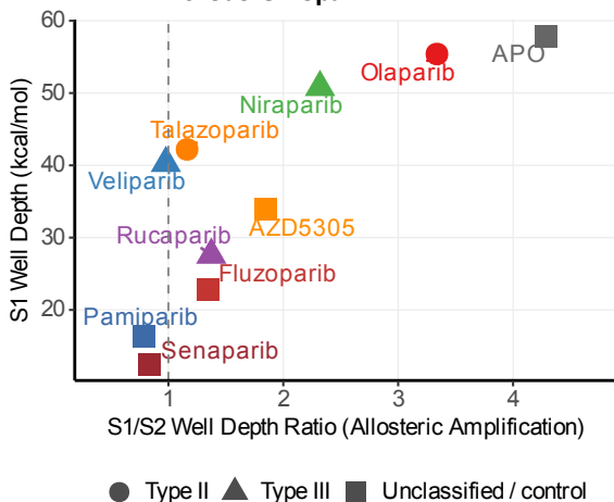
C AAI versus S1 span
