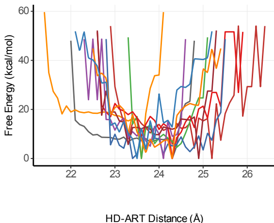
A S1: CAT-only HD-ART Free Energy Landscape
