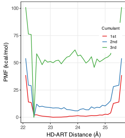
Veliparib (Type III)
