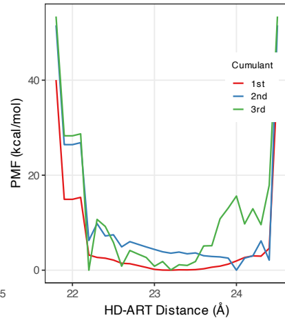
Rucaparib (Type III)
