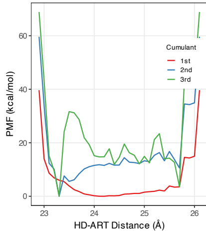
Olaparib (Type II)
