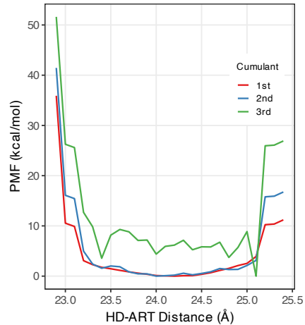
Niraparib (Type III)
