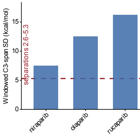
A Window noise vs between-system separations
